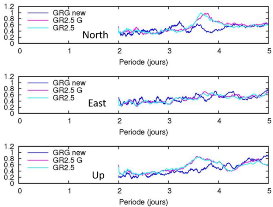
Figure 2: Lomb-scargle normalized periodogram of new GRG and old GRG2.5G (GPS only) and old GR2.5 (GPS+GLONASS) solutions. The spurious 3.7 day period signal affecting the Up and North components seems to disappear when using the new strategy.
