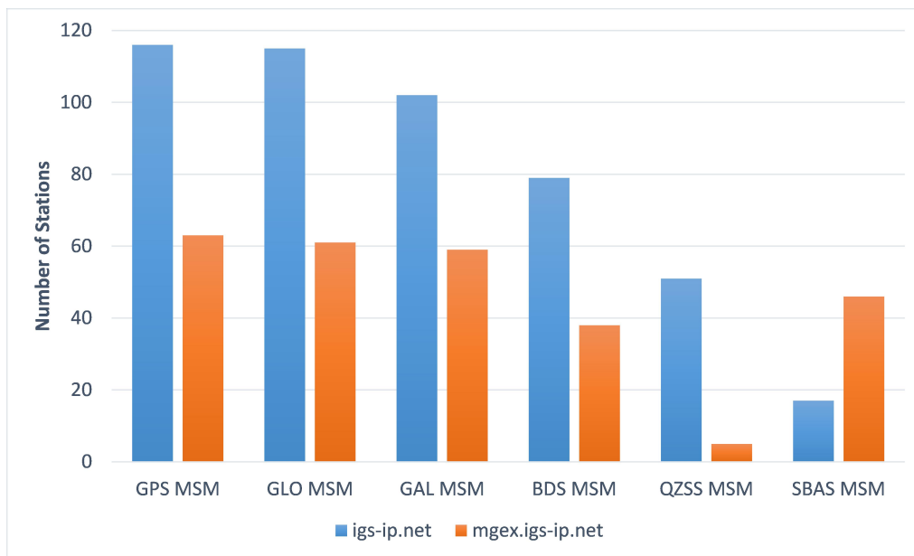
Figure 5: Number of stations broadcasting RTCM3 Multi-Signal-Messages for different GNSS constellations. Streams at the BKG IGS-caster are receiver generated, streams at the BKG MGEX-caster are software generated.
