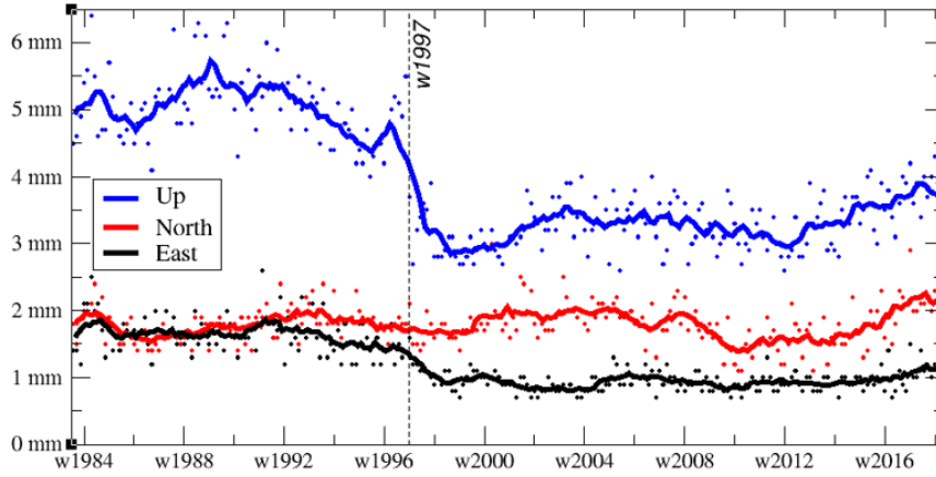
Figure 1: Station daily comparison: GRG vs IGS combined solution. The change of processing strategy during week 1997 has a clear positive impact on the GRG solution (Courtesy Paul Rebischung, IGN, France).
