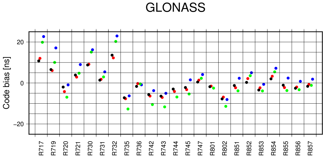
Figure 2: Observable-specific code bias (OSB) estimates for GLONASS code observable types (using the RINEX3 nomenclature) and GLONASS SV numbers, computed at CODE, for January 2019. Note that R717–R747 and R851–R857 correspond to GLONASS-M; R801–R802 correspond to GLONASS-K1 satellite generations.
