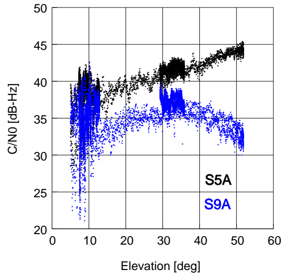
Figure 2: Carrier-to-noise-density ratio for IRNSS L5 (S5A) and S-band (S9A) tracking of the IGS station Ganovce (GANP00SVK).
