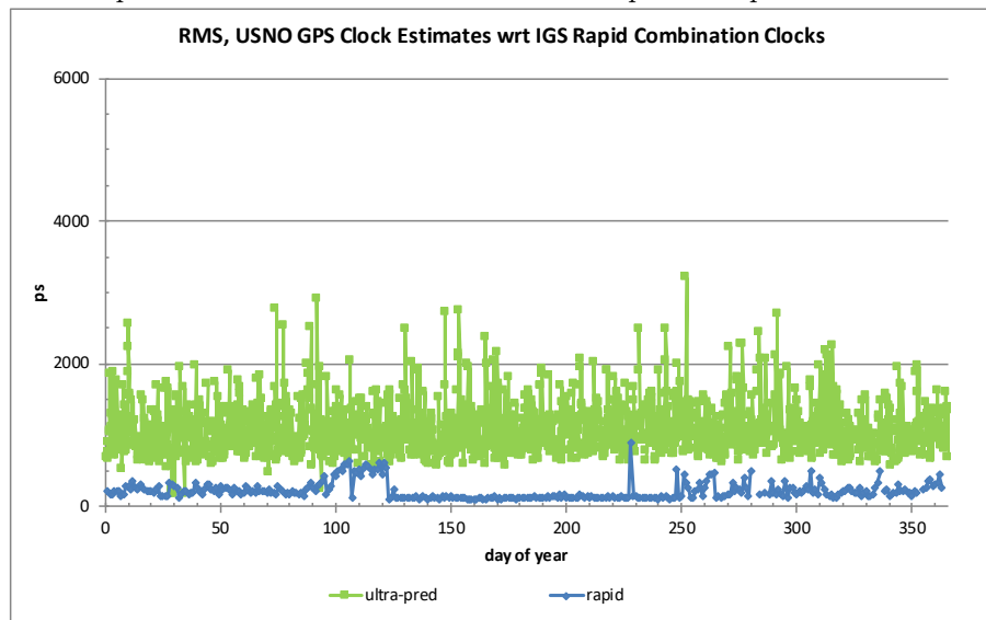
Figure 2: RMS of USNO GPS rapid clock estimates and Ultra-rapid clock predictions with respect to IGS Rapid Combination, 2018.
