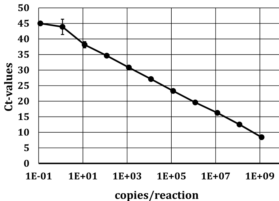
Figure 1. qRT-PCR standard curve of in vitro transcribed APPV RNA in the 5'UTR. A tenfold dilution series within a range of 1 \times 10^9 molecules/reaction to 1 \times 10^{-1} molecules/reaction was performed. Targeting the FAM reporter, an efficiency of 86.5% was achieved. The slope of the standard curve was -3.7 with a standard deviation (SD) between 1 and 2.5.
