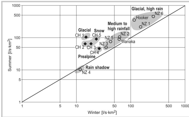
FIGURE 9 Half-year summer (CH, April–September; NZ, October–March) versus winter-specific mean flows for the representative catchments of the Swiss and Southern Alps, including flows of the Hooker River and from Lake Wanaka for the Southern Alps.
