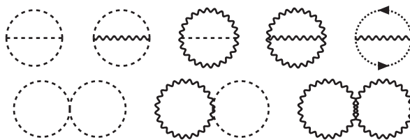
Figure 10. 2-loop topologies contributing to the 3d V_{\text{eff}} , in Landau gauge. Sunset-type diagrams on the first row are divergent in the UV and exactly determine the RG evolution of the mass parameters in the 3d EFT.
