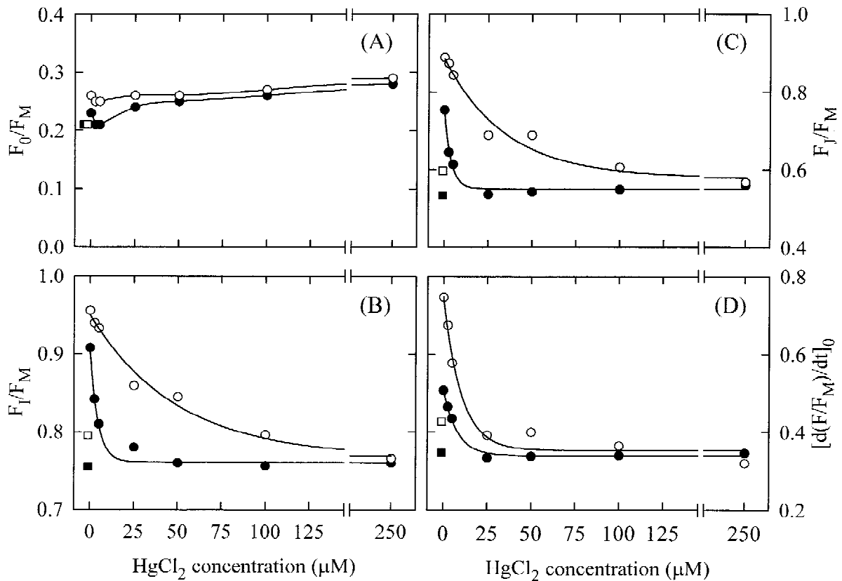
Figure 5. Effects of different concentrations of HgCl 2 on the selected parameters (see legend of Figure 2) characterising the fluorescence rise kinetics, calculated from the fluorescence transients obtained from osmotically broken spinach chloroplasts that were incubated for 60 min at room temperature in the dark in the presence of 500 μM NADPH. The experiment was conducted both under aerobic (●) and anaerobic (○) conditions. The detached symbols (■ for aerobic and □ for anaerobic conditions) correspond to samples where neither NADPH nor HgCl 2 were added (control samples).
