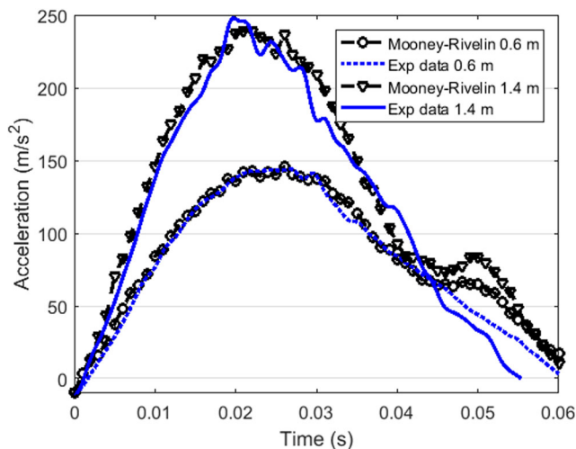
Fig. 6 Acceleration data of the impactor for a height of 0.6 m corresponding to impact energy of 12 J and a height of 1.4 m corresponding to an energy of 28 J compared to the Mooney-Rivlin model using the mechanical parameters proposed by Liu et al. [18]
