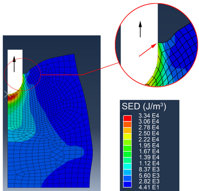
Fig. 7 Axisymmetric model of the impactor retreating from the gelatin at 0.05 s (black arrow indicates direction). Impact energy E = 36 J. The gelatin block shows the chosen mesh with the SED distribution. Enlarged: Section showing the interface between the impactor and the gelatin with the gelatin sticking to the impactor (red arrow)
