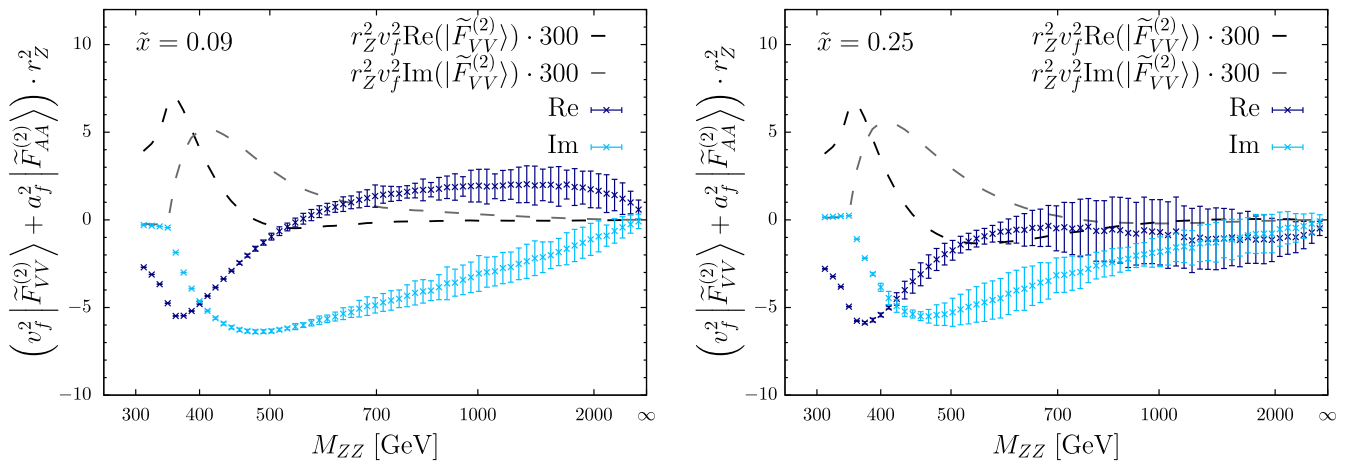
FIG. 6. The interference form factor v_f^2 |\tilde{F}_{VV}^{(2)}\rangle + a_f^2 |\tilde{F}_{AA}^{(2)}\rangle for \tilde{x} = 0.09 (left side) and \tilde{x} = 0.25 (right side) as a function of the invariant mass of the Z-boson pair. The dashed lines show a rescaled form factor |\tilde{F}_{VV}^{(2)}\rangle to demonstrate that it is negligible compared to |\tilde{F}_{AA}^{(2)}\rangle .
