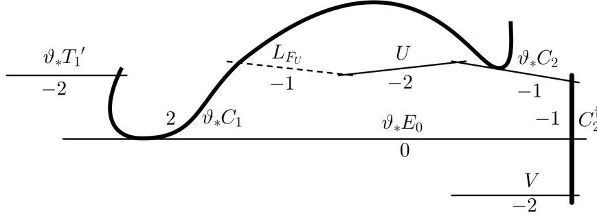
FIGURE 22. The \mathbb{P}^1 -fibration from Remark 4.15(a).
