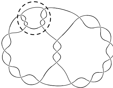
FIGURE 1. A prime knot K with g_4^{\text{top}}(K) = 0 , g_{\text{alg}}(K) > 0 , g_4(K) > 0 (drawn with knotscape [12]).
