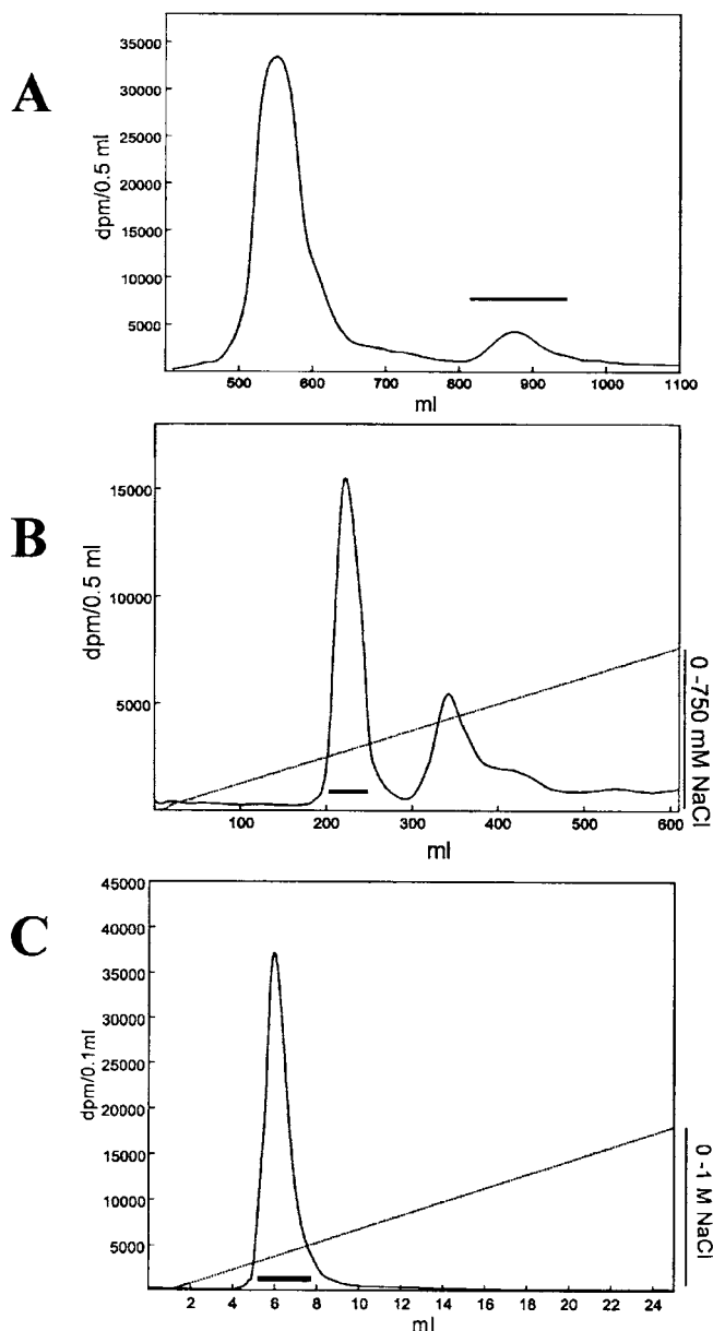
FIG. 1. Elution of \alpha -[ ^3\text{H} ]tocopherol on Sephacryl S-200 gel filtration (A), Affi-Gel Blue affinity chromatography (B), and ion exchange chromatography (C). The horizontal bars indicate pooled fractions used for further purification. Broken lines show salt gradients. See "Experimental Procedures" for details.
