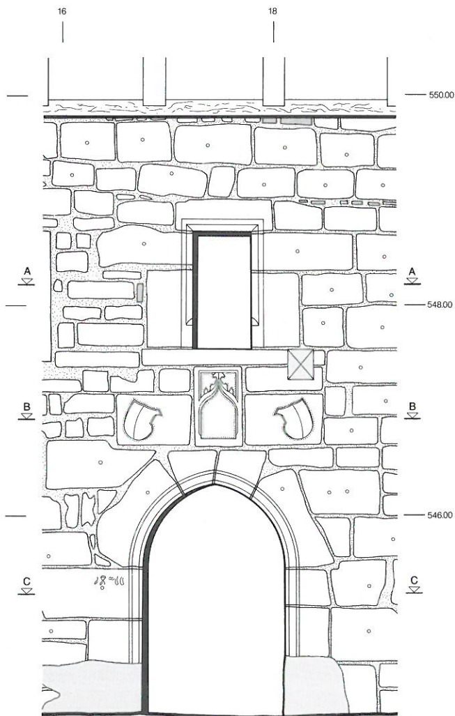
Abb. 10: Portalsituation (1:50).
