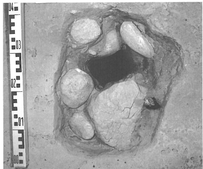
Abb. 6: Detail Pfostenloch.
