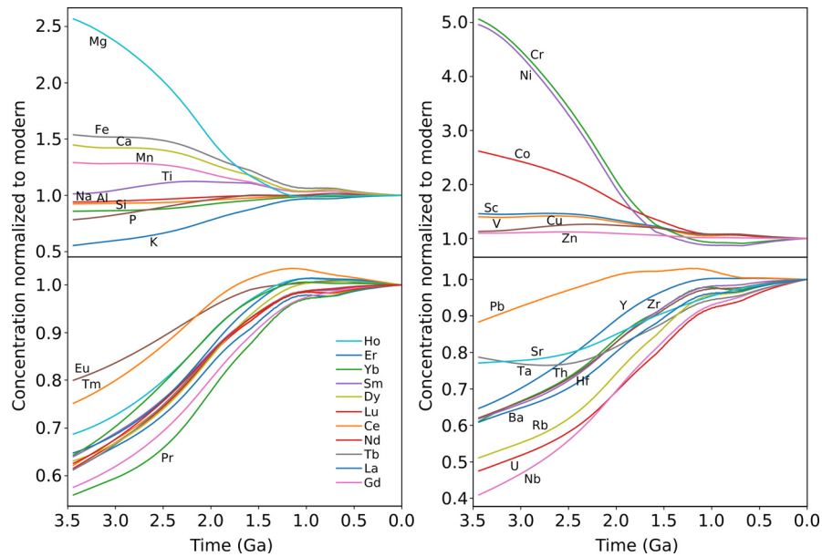
Fig.6. Reconstructed concentrations of selected elements through time in the Earth's upper continental crust normalized to calculated modern-day values. This reconstruction used the best eight-ratio combination, thereby using as much information as possible to obtain the most robust result. The concentration of Si in the upper crust increased from 61% to 66% since 3.5 Ga, indicating that despite the observed changes in the concentrations of many major, trace, and rare earth elements, the crust has remained predominantly andesitic over the last 3.5 billion years. The main driver of change in elemental concentrations is the changing composition of both mafic and felsic rocks through time (due to the secular cooling of the Earth) and the greater proportion of komatiites in the Archaean, rather than a change in the relative proportions of felsic and mafic material.
