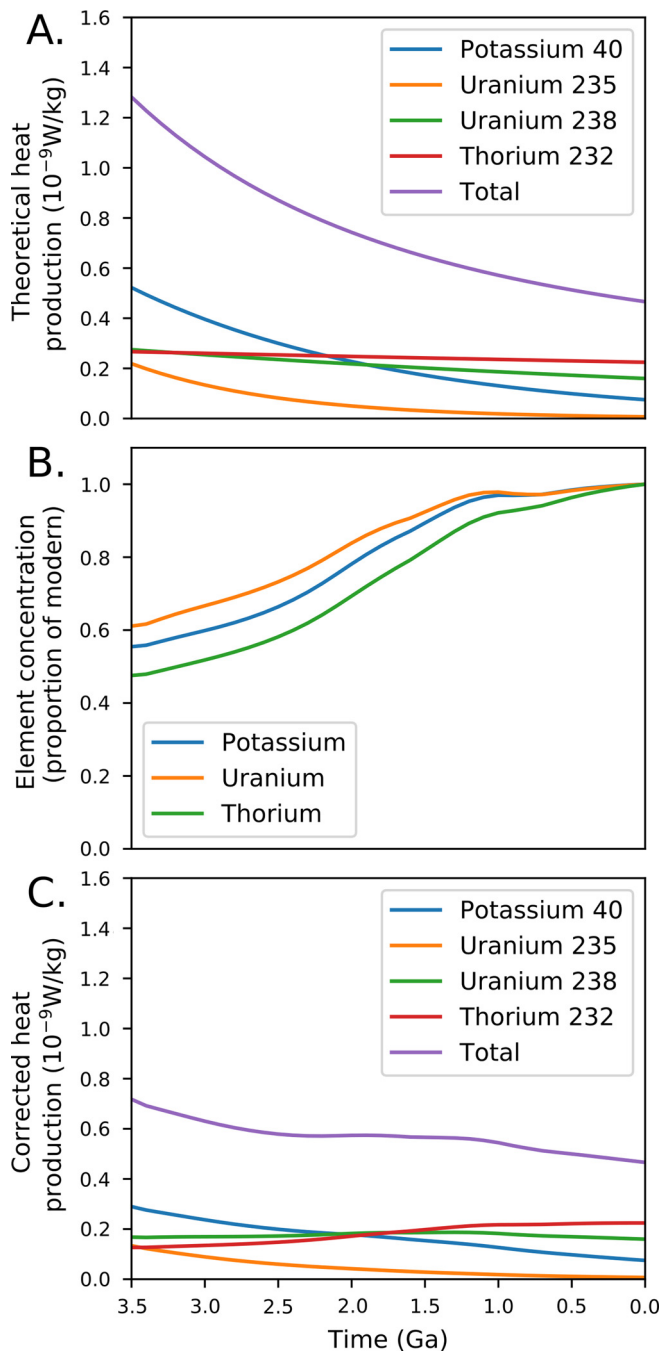
Fig.8. Changes in crustal radiogenic heat production through time. (a) Predicted contributions of K, Th, and U to crustal heat production, in a hypothetical scenario where their crustal concentrations remained constant through time. (b) Relative changes in the concentrations of these elements through time normalized to the present-day values, as predicted by our reconstruction. (c) Our estimate of actual crustal radiogenic heat generation based on the changes in concentration given by our reconstruction, constructed by multiplying (a) with (b). Note that the amount of heat produced by radioactive elements in the continental crust is predicted to have decreased by around 50% over the last 3.5 Ga.
