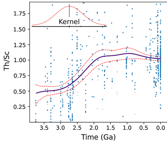
Fig.2. Example output of the bootstrap algorithm when applied on filtered sedimentary Th/Sc (ppm/ppm) data. Red dotted line represents 95% confidence intervals, thick black line the best fit. The model used was a moving average with a Gaussian kernel of 400 Myr bandwidth (see inset). The blue points are sediment measurements which have been accepted by the LOF filter – grey points have been rejected.
