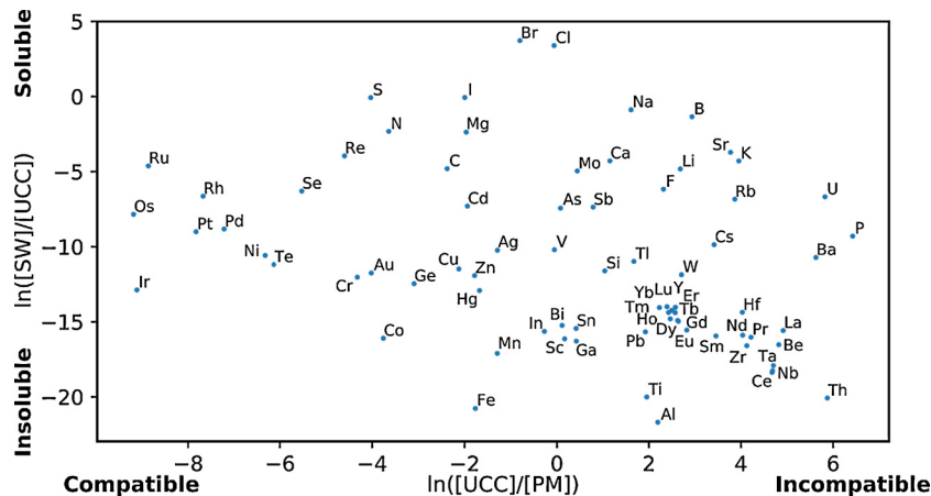
Fig.3. Metrics of solubility in aqueous medium against igneous compatibility for most naturally-occurring elements. Solubility is roughly quantified as the natural logarithm of the ratio of the elemental concentration in seawater (SW) to that in the upper continental crust (UCC). Igneous compatibility is quantified as the logarithmic ratio of UCC to primitive mantle (PM) concentrations. The ideal combination of proxies for reconstructing the continental crust will contain elements that are insoluble and span a wide range of igneous compatibility. Such a combination will make it easy to distinguish between komatiite, mafic, and felsic rocks. See text for a more in-depth discussion of element suitability. Primitive mantle concentration data from McDonough and Sun (1995); upper continental crust data from Wedepohl (1995); average seawater concentrations from Bekov et al. (1984), Nozaki (1997), and Sohrin et al. (1998).
