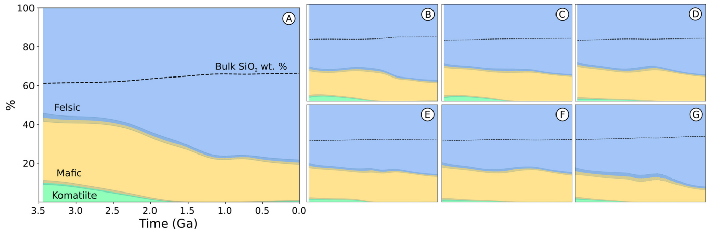
Fig.5. Reconstructed contribution of felsic, mafic, and komatiitic material to the upper continental crust as a function of time, according to several different systems of proxy ratios. (A) The best eight-ratio system \text{Al}_2\text{O}_3/\text{La} , \text{Ce}/\text{Y} , \text{Co}/\text{Ni} , \text{Cr}/\text{Yb} , \text{Hf}/\text{TiO}_2 , \text{Nb}/\text{Pb} , \text{Sc}/\text{Zr} , \text{Ta}/\text{Th} . (B) The best seven-ratio system \text{Al}_2\text{O}_3/\text{La} , \text{Ce}/\text{Y} , \text{Co}/\text{Ni} , \text{Cr}/\text{Yb} , \text{Hf}/\text{TiO}_2 , \text{Sc}/\text{Zr} , \text{Ta}/\text{Th} . (C) The best six-ratio system \text{Al}_2\text{O}_3/\text{TiO}_2 , \text{Co}/\text{Ni} , \text{Cr}/\text{Yb} , \text{La}/\text{Y} , \text{Sc}/\text{Zr} , \text{Ta}/\text{Th} . (D) The best five-ratio system \text{Al}_2\text{O}_3/\text{TiO}_2 , \text{La}/\text{Yb} , \text{Ni}/\text{Y} , \text{Sc}/\text{Zr} , \text{Ta}/\text{Th} . (E) The best four-ratio system \text{Al}_2\text{O}_3/\text{TiO}_2 , \text{Ni}/\text{Yb} , \text{Sc}/\text{Zr} , \text{Ta}/\text{Th} . (F) The best three-ratio system \text{Al}_2\text{O}_3/\text{TiO}_2 , \text{Ni}/\text{Y} , \text{Sc}/\text{Zr} . (G) The best two-ratio system \text{Ni}/\text{TiO}_2 , \text{Sc}/\text{Zr} .
