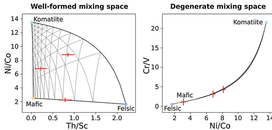
Fig.4. Illustration of our approach to find the best-formed mixing space (Sect.2.5; Table1). We performed an exhaustive search of all possible combinations of selecting n ratios from a set of 16 elements (Sc, Cr, Co, Ni, Pb, Zr, Hf, Nb, Ta, Ti, Al, La, Ce, Yb, Y, and Th) for values of n between 2 and 8. For each mixing space, we input three synthetic test points, with variances (shown as red crosses) corresponding to the real-world variances of those ratios in our sedimentary database. We then run our reconstruction algorithm on these synthetic test points, using real endmember compositions, and calculate how accurately the rock proportions are recovered by the inversion. In the degenerate example (right), even small uncertainties in the synthetic test points lead to a large deviation in the predicted endmember contributions. The well-formed system (left) is ranked 21/5460 by the algorithm.
