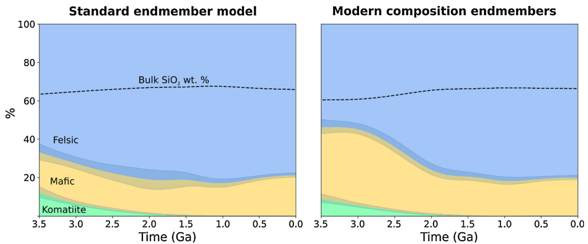
Fig.7. The results of running a Th/Sc + Ni/Co reconstruction with our time-variant endmember model (left), and with a time-invariant endmember model based only on modern rocks, effectively ignoring the changes in the composition of igneous rocks over the last several billion years (right). Ignoring this change in the composition of igneous rocks introduces a strong bias towards mafic in the Archaean.
