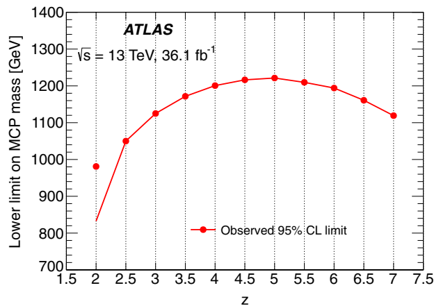
FIG. 9. Observed 95% C.L. lower mass limits of leptonlike MCPs for charges z \in [2, 7] with a Drell-Yan pair-production model. The mismatch between the left end of the continuous line and the marker at z = 2.0 (a shift by 150 GeV) is due to the difference in efficiencies between the cases where the z = 2 and z > 2 selections are applied to the z = 2.0 samples, making this line segment constitute a conservative mass limit for 2.0 < z < 2.5 particles.
