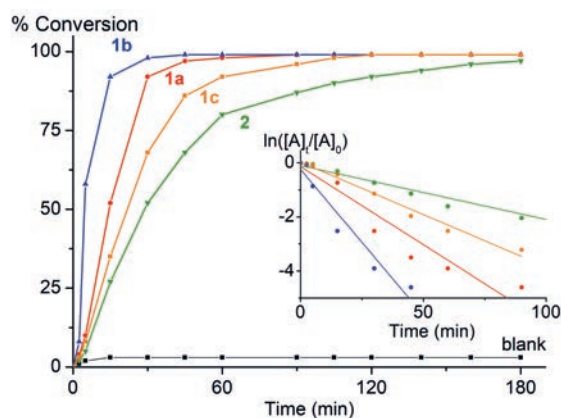
Fig. 2. Hydrosilylation of 4-methylbenzaldehyde with complexes 1a–c and 2 . Inset: linear correlation of the time (min) with \ln([A]_t/[A]_0) for each catalyst, [\ln([A]_t/[A]_0)] = -k \text{ time} , R^2=0.99 (green line), 0.98 (orange line), 0.93 (blue line) and 0.92 (red line).
