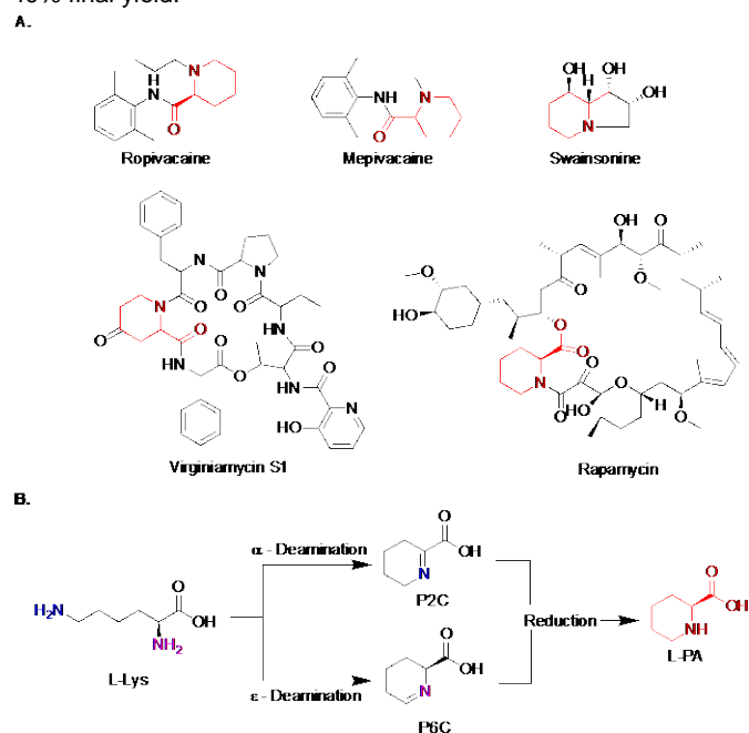
Figure 1. A. Chemical structures of L-PA containing drugs (L-PA identified in red). B. General reaction scheme of the biosynthetic pathway for the production of L-PA.
