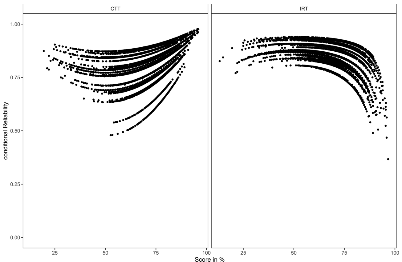
Fig. 1 Mean conditional reliability and standard deviation in classical test theory (CTT) and item response theory (IRT) calculated over 32 exams
