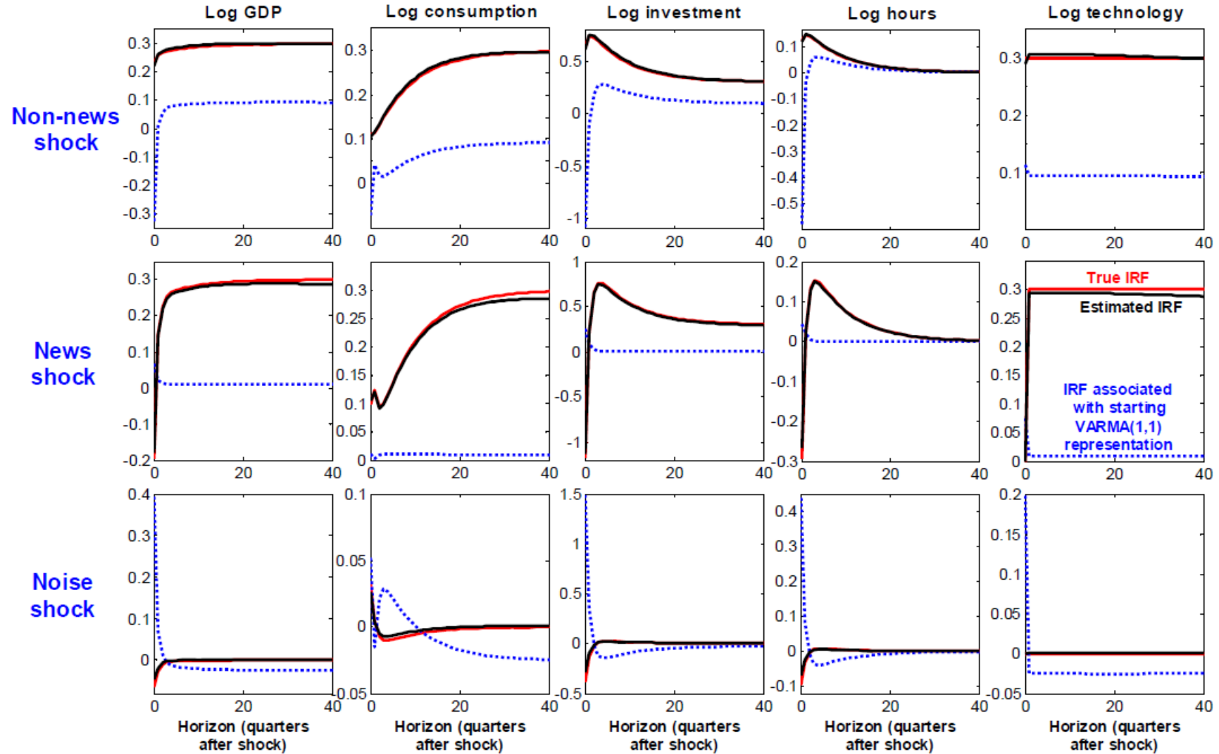
Figure 3 Recovering news and noise shocks in population: Theoretical IRFs, and estimated IRFs based on the theoretical truncated VARMA(1,1) representation of the RBC model augmented with noise shocks about TFP
