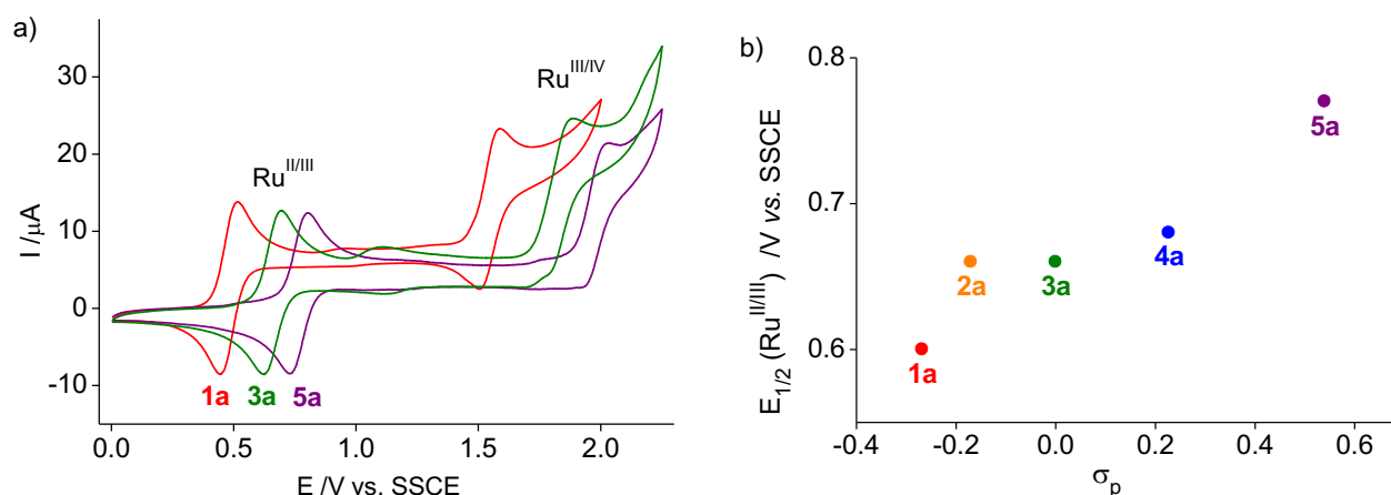
Figure 2. a) Cyclic voltammometry measurements of complexes 1a (red), 3a (green), and 5a (purple) in MeCN (1 mM complex conc., potentials vs. SSCE using the \text{Fc}^+/\text{Fc} couple as standard; E_{1/2} = +0.4319 and n\text{-Bu}_4\text{NPF}_6 as electrolyte, 100 \text{ mVs}^{-1} scan rate). b) Redox potentials vs. \sigma_p for complexes 1a–5a .
