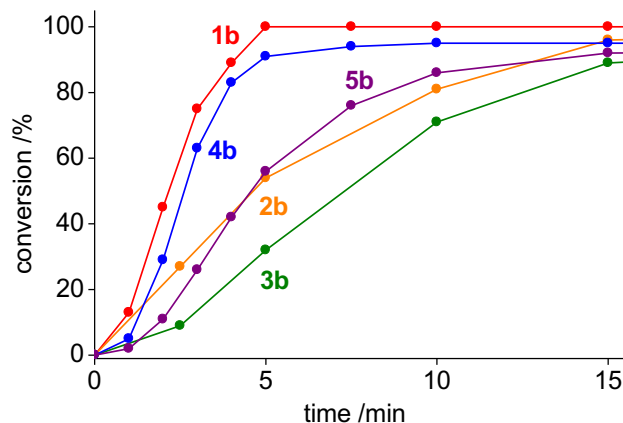
Figure 7. Time-conversion profiles for the transfer hydrogenation of benzophenone with in situ formation of \text{PPh}_3 -complexes after pre-activation of the complex in the presence of 2 moleq. \text{PPh}_3 for 10 min at 70^\circ\text{C} , 1b (red), 2b (yellow), 3b (green), 4b (blue) and 5b (purple). Reaction conditions: benzophenone (5.0 mmol), KOH (0.05 mmol, 1 mol%), cat. (0.005 mmol, 0.1 mol%), \text{PPh}_3 (0.01 mmol, 0.2 mol%) i PrOH (10 ml), \text{N}_2 atm., reflux temperature.
