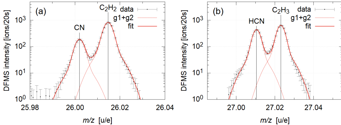
Figure 1. Typical spectra at integer masses m/z = 26 u/e (a) and 27 u/e (b) collected at the beginning of the Rosetta mission phase on 17 th September 2014 over the southern hemisphere of comet 67P. Both the CN as well as the HCN signals are clearly separated from the signals of C_2H_2 and C_2H_3 respectively. Error bars indicate only the statistical error.
