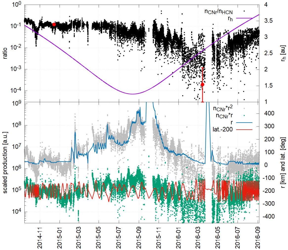
Figure 4. (top) Full mission lower limit local density of CN relative to the local density of HCN as n_{\text{CNr}}/n_{\text{HCNr}} (black dots). The heliocentric distance r_h is indicated as purple line. The relative statistical errors of the density ratio vary between a few per cent (mid-December 2014, where n_{\text{CNr}} and n_{\text{HCNr}} are of the same order of magnitude) and more than 500 per cent (mid-March 2016, where n_{\text{CNr}} and n_{\text{HCNr}} differ by almost four orders of magnitude). Two indicative error bars are shown in red: 4 per cent on 14 th December 2014 (smaller than symbol size) and 502 per cent on 15 th March 2016. Systematic errors of about 5 per cent must be considered in addition. (bottom) n_{\text{CNr}}*r^2 (gray dots) and n_{\text{CNr}}*r (green dots) versus time. Note that the overlaid cometocentric distance r (blue line) is shown on a linear scale together with the sub-spacecraft latitude (red line), offset by -200 deg. 30 per cent total error bars on n_{\text{CNr}} have been omitted for visual clarity.
