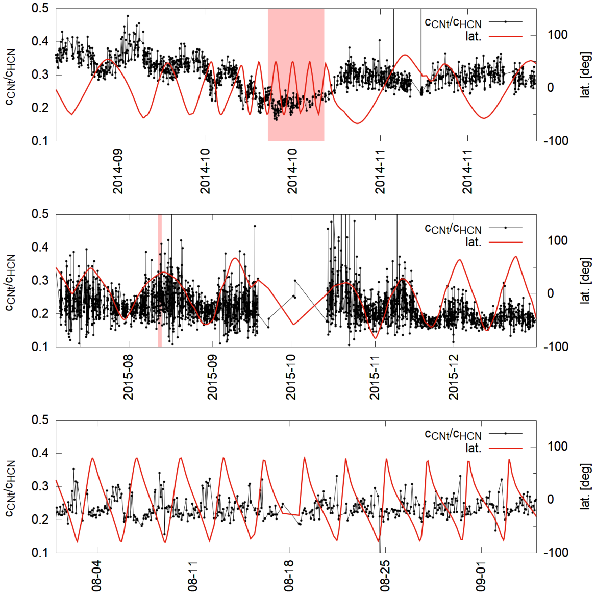
Figure 3. The \text{CCNt}/\text{CHCN} ratio at the beginning of the Rosetta mission phase (top), around perihelion (middle) and during the end-of-mission elliptical orbits from early August to early September 2016 (bottom). The latitudinal position of the spacecraft above the cometary surface is shown with a red line. The 10 km-orbital phase (15 th to 28 th October 2014) and the date of the perihelion (13 th August 2015) are shaded in pink. 10 per cent error bars on \text{CCNt}/\text{CHCN} have been omitted for visual clarity.
