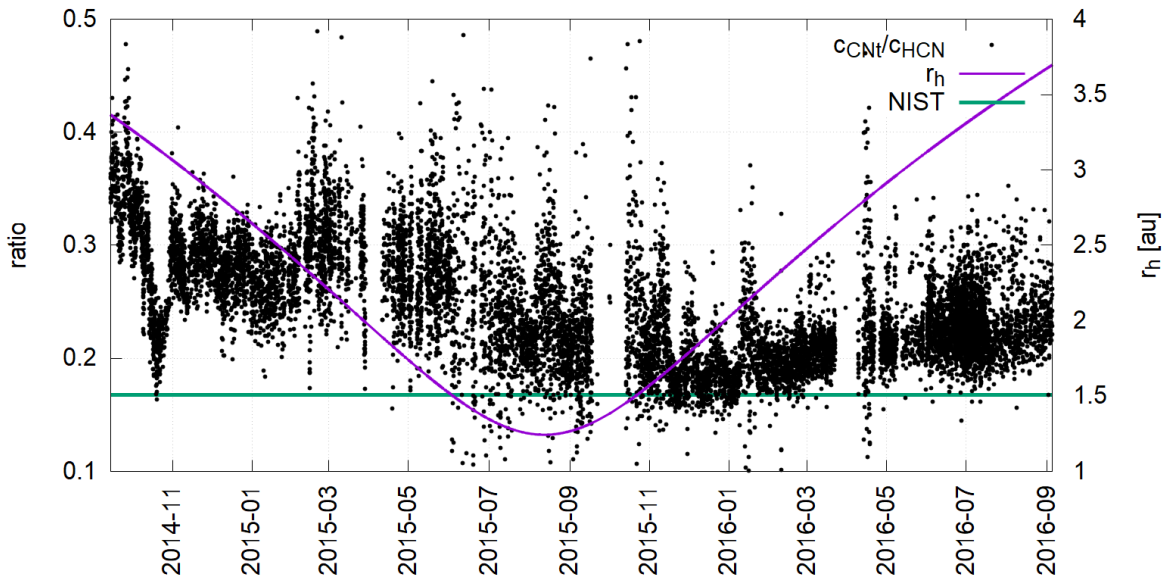
Figure 2. \text{CCNt}/\text{CHCN} ratio from nadir-corrected MCP row A full-mission data. The green line indicates the expected constant CN signal relative to HCN (NIST value) due to the fragmentation of the latter under EI inside the ion source, i.e. \text{CCNf-HCN}/\text{CHCN} . The purple line indicates 67P's heliocentric distance r_h . Error bars on \text{CCNt}/\text{CHCN} have been omitted for visual clarity.
