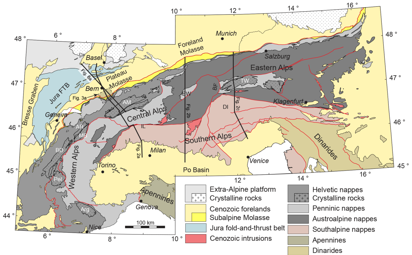
Figure 1. Tectonic map of the European Alps and its foreland basins (adapted from Schmid et al., 2004). Traces of the cross sections in Figs. 2 and 8a are given as bold black lines. The sample area south of Bern (Fig. 3a) is denoted by a dashed rectangle. AM, Aar Massif; AR, Aiguilles Rouges Massif; BD, Belledonne Massif; BF, Brenner Fault; DI, Dolomite indenter; EW, Engadine Window; FTB, fold-and-thrust belt; IL, Insubric Line; MB, Mont Blanc Massif; Pel, Pelvoux Massif; TW, Tauern Window.
