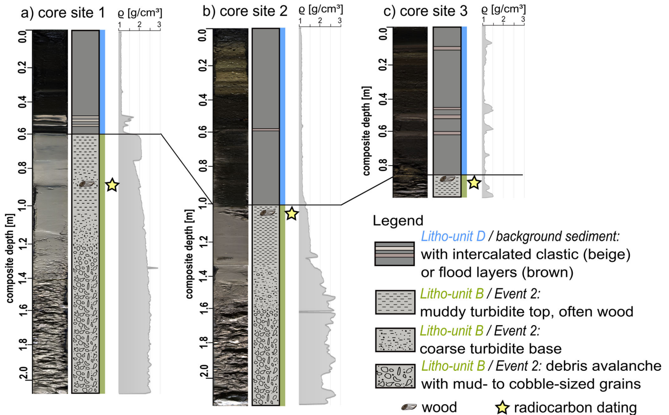
Figure 4. Core-to-core correlation with photographs, sedimentological descriptions, and density profiles at locations 1, 2, and 3 in the western and middle parts of the lake.
