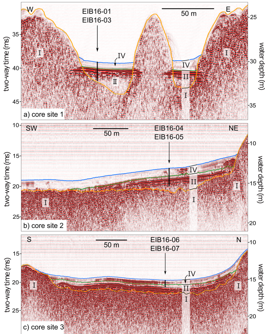
Figure 3. Seismic profiles at core sites 1, 2, and 3 (see Figure 1b for locations). Seismic units as in Figure 2.
