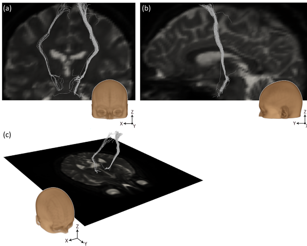
Figure 4. Streamlines from the right and left STN in subject 1, ending in the motor cortex, that do not pass through thalamus, caudate, putamen or globus pallidus. These streamlines are therefore an indication for the existence of the “hyperdirect” pathway. (a) Coronal view. (b) Sagittal view on streamlines from the right STN. (c) Streamline rendering in 3D, showing an axial plane of the unweighted diffusion image. doi:10.1371/journal.pone.0039061.g004
