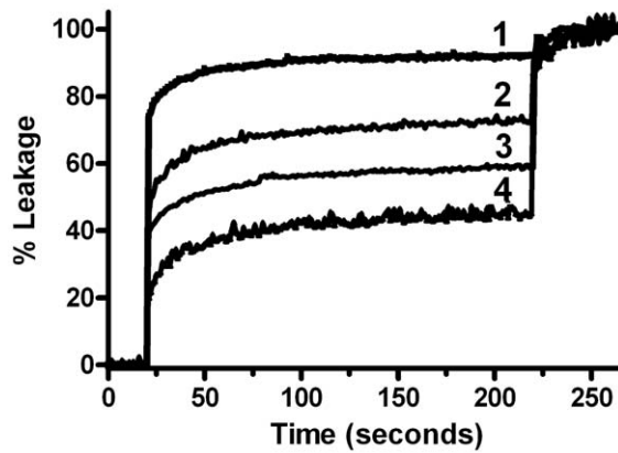
Figure 5. Phosphocreatine and creatine protect lipid vesicles against melittin-induced permeabilization. 50 \mu M of CH/POPE/POPC/SP-LUVs entrapping a quenched ANTS/DPX solution were injected into PIPES buffer (20 mM pH 7.4, isomolarity of the entrapped solution was adjusted to be equal to that of the external media with NaCl). The media external to the liposomes contained only phosphate buffer and NaCl (trace 1) or 100 mM DMBG (trace 2), Cr (trace 3), or PCr (trace 4). Leakage was begun with 500 nM melittin. All buffers and entrapped ANTS/DPX solution were adjusted to the same osmolarity and each compound was tested twice. Fluorescence dequenching was followed at 530 nm and normalized to the signal obtained after full permeabilization of LUVs. doi:10.1371/journal.pone.0043178.g005
