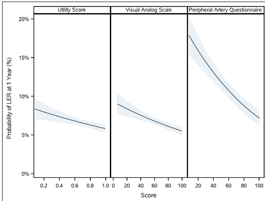
Figure 3. Association of baseline EQ-5D index score, EQ-5D VAS, and PAQ scores and risk of LER. There is a significant association between the baseline EQ-5D index score, EQ-5D VAS, and the PAQ scores and the 1-year probability of LER. EQ-5D indicates EuroQol 5-Dimensions; LER, lower-extremity revascularization; PAQ, peripheral artery questionnaire; VAS, visual analog scale.
