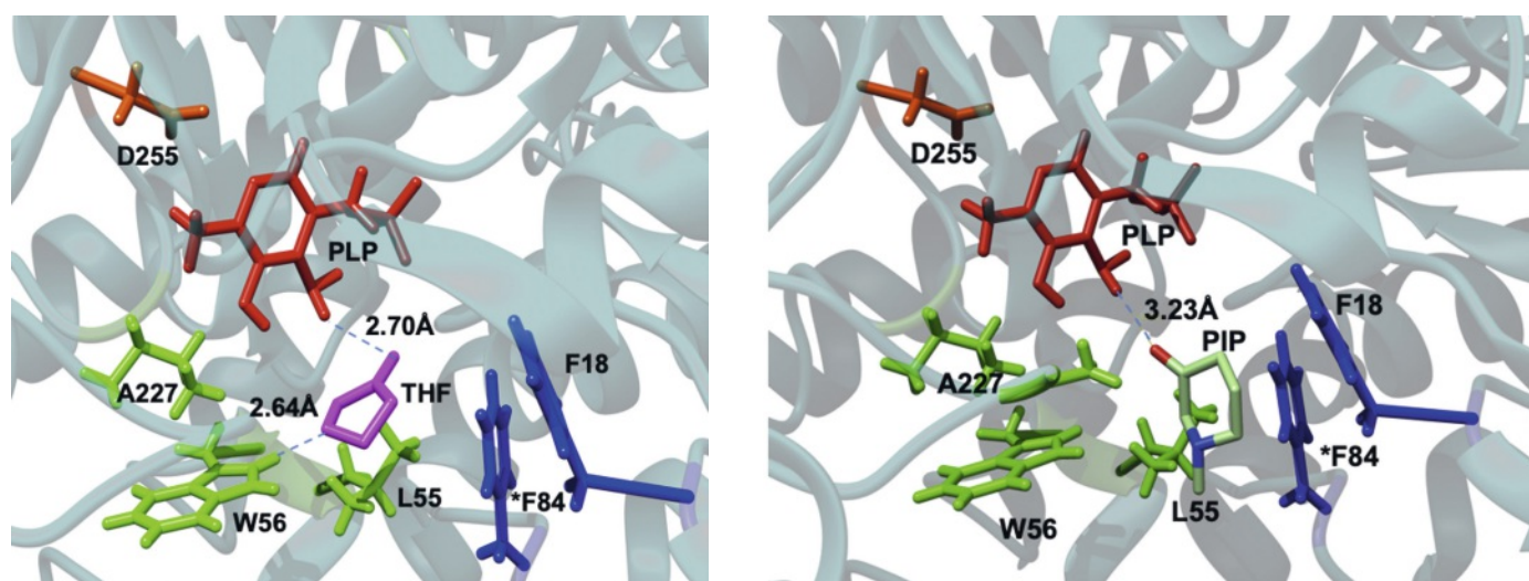
Fig. 1. Docking poses for tetrahydrofuran-3-one (left) and 1-methyl-3-piperidinone (right) in the active site of HeWT (PDB: 6GW1). Figures were generated using Chimera.
