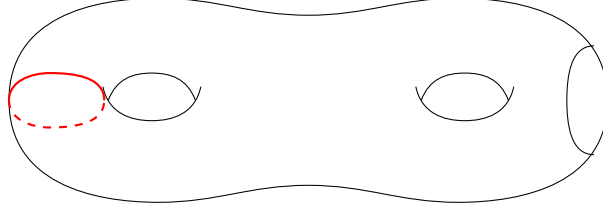
Figure 2: \gamma_1
