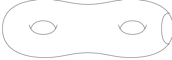
Figure 1: \mathbb{T}^2 \# \mathbb{T}^2 \setminus D
