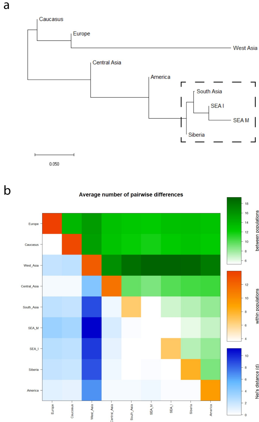
Fig 1. a) The Neighbour-Joining (NJ) tree showing the genetic relationship of the studied populations. The figure was drawn from the Fst distances obtained from the haplotype analysis of Eurasian populations. b) Heat map showing the intra- and inter-population variation measured by average pairwise sequence differences of the ACE2 gene. The average pairwise differences between populations are shown in the upper triangle of the matrix (green). The average number of pairwise differences within each population group are shown along the diagonal (orange). The differences between populations based on Nei's genetic distances are depicted in lower triangle of the matrix (blue). The obtained values of various parameters have been shown at the color scales.
