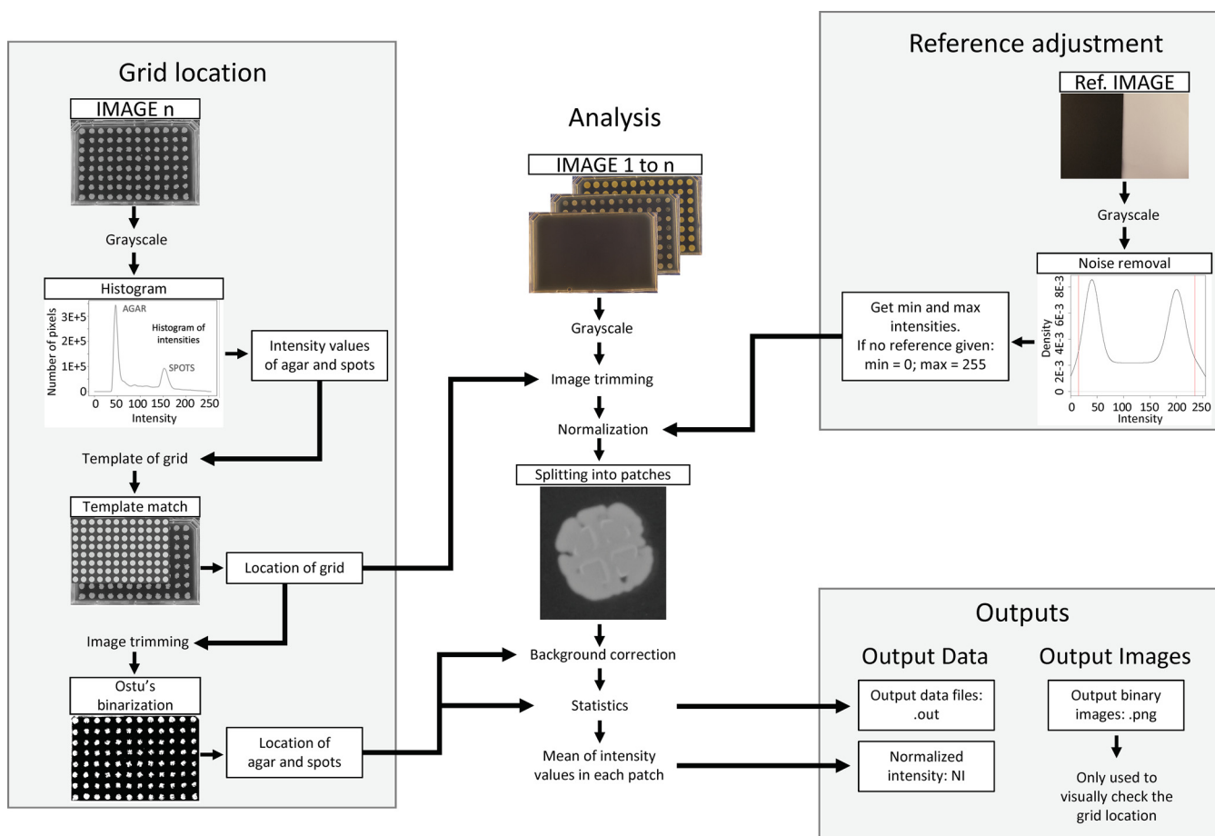
FIG 2 Conceptual design of the BaColonyzer algorithm, described in more detail in Text S1.
