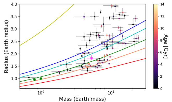
Figure 8. Mass–radius diagram of all planets smaller than 4R_\oplus with a mass measurement significance better than 3\sigma (using data from the NASA exoplanet archive accessed 2020 June 11). The points are colour-coded according to their stellar host ages (in case no age was determined, the point is black). The green dots bottom left represent Venus and Earth, respectively. The solid lines show planetary interior models for different compositions, top to bottom: Cold H_2/He , 100 per cent H_2O , 50 per cent H_2O , 100 per cent MgSiO_3 , 50 per cent Fe, and 100 per cent Fe. The larger magenta square represents K2-111 b.
