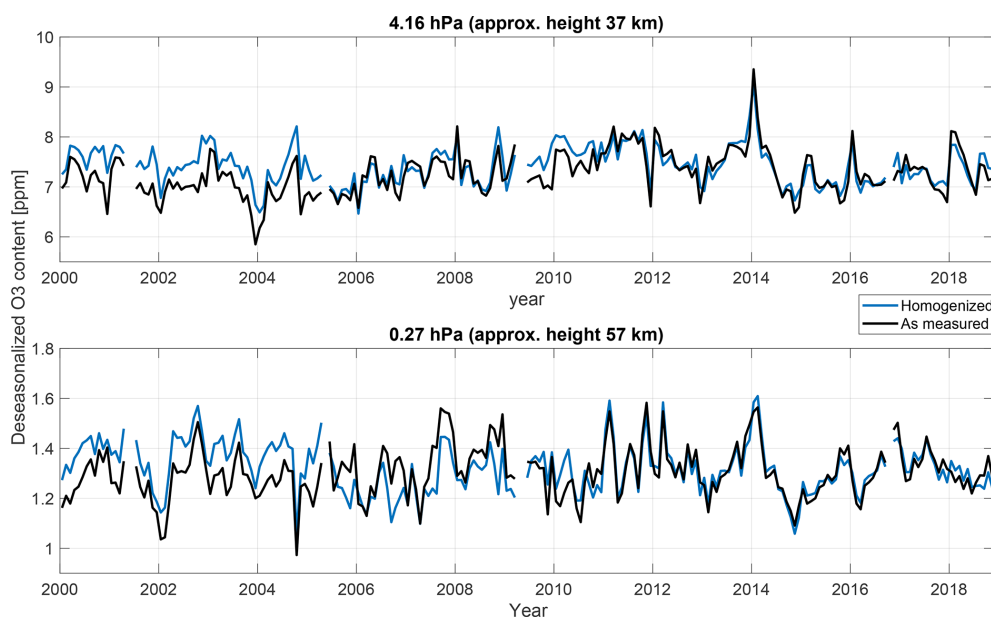
Figure 4. Deseasonalized ozone monthly mean time series before (in black) and after (in blue) the homogenization for a representative layer in the middle stratosphere and in the low mesosphere.
