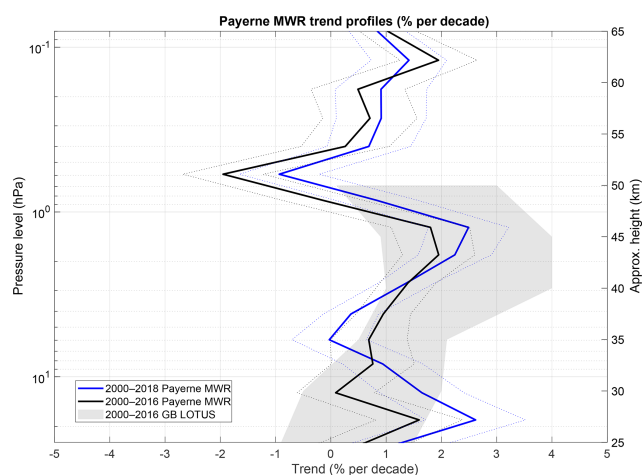
Figure 7. Payerne MWR O 3 trend profiles for the 2000–2016 time range in black and 2000–2018 time range in blue. The dotted lines show the 2 \sigma uncertainties. The shaded area is the full range of LOTUS ground-based 2000–2016 trend profiles.
