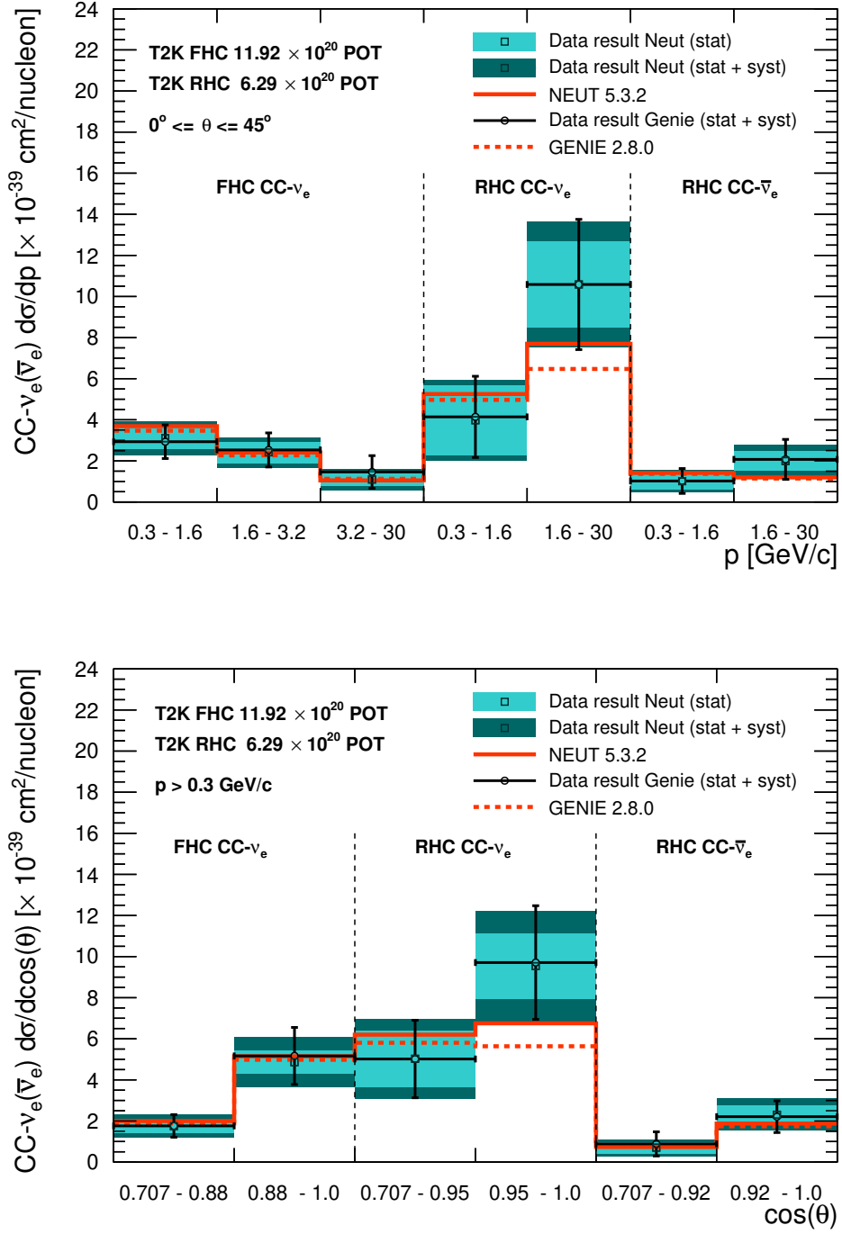
Figure 17. CC-\nu_e and CC-\bar{\nu}_e inclusive cross-section results in d\sigma/dp (top) and d\sigma/d\cos(\theta) (bottom) in a limited phase-space ( p > 300 \text{ MeV}/c and \theta \leq 45^\circ ). The statistical uncertainty is computed by fixing all the nuisance parameters to their post-fit nominal values and redoing the fit. The systematic uncertainty is computed by subtracting in quadrature the statistical uncertainty from the total uncertainty.
