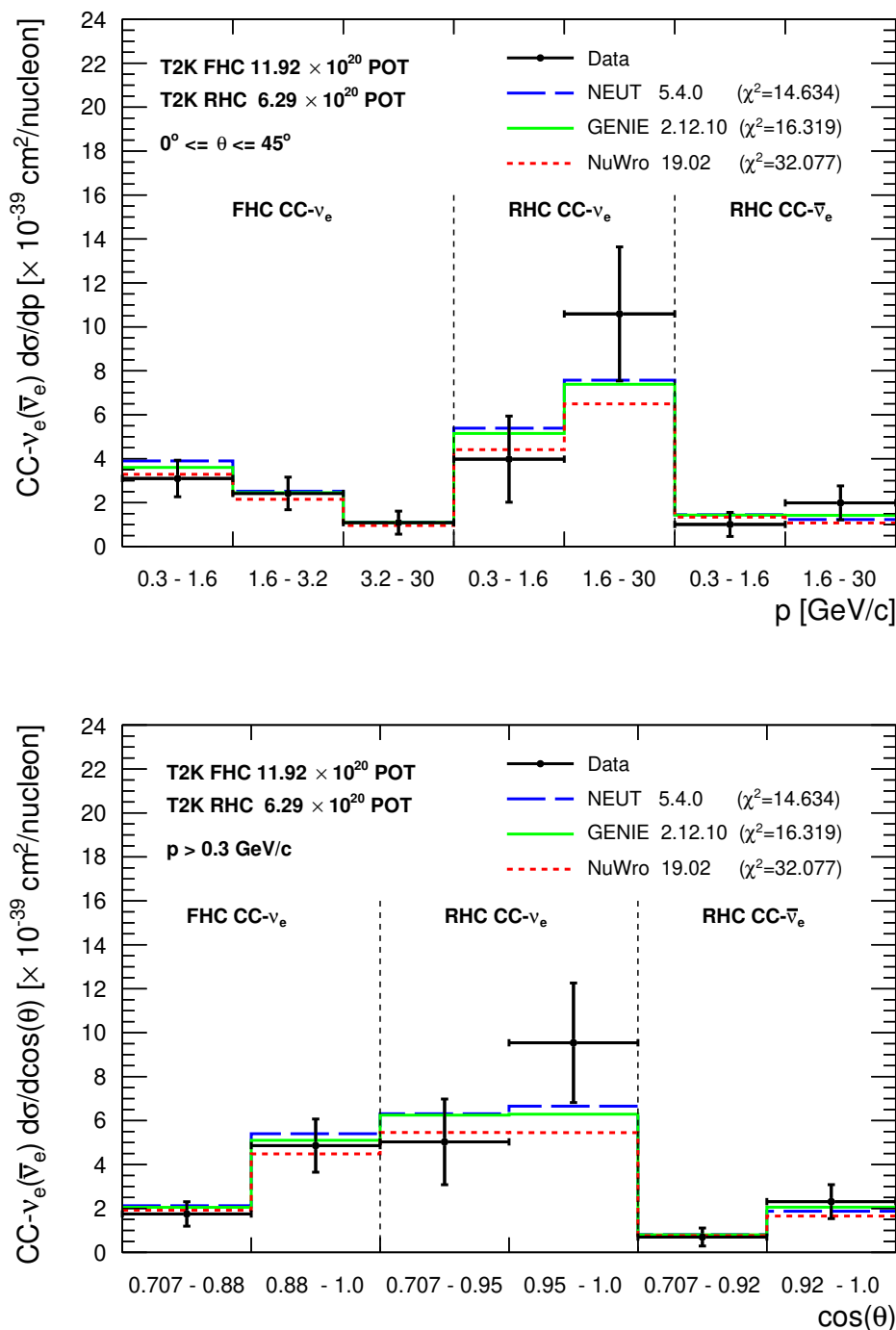
Figure 19. Flux integrated CC-\nu_e and CC-\bar{\nu}_e inclusive cross-section results in a limited phase-space ( p > 300 MeV/c and \theta \leq 45^\circ ) with comparisons to neutrino generator models from NEUT 5.4.0, GENIE 2.12.10 and NuWro 19.02 obtained using the NUISANCE framework. The top plot shows the results in momentum and the bottom plot the results in scattering angle. The \chi^2 is the total from the combined measurements in momentum and \cos(\theta) .
