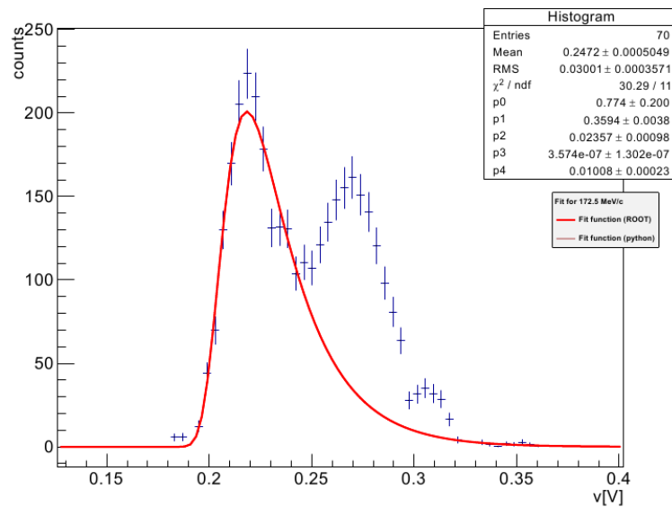
Figure 5. Spectrum of energy loss measured by the thick detector of the telescope at momentum 172 MeV/c.
