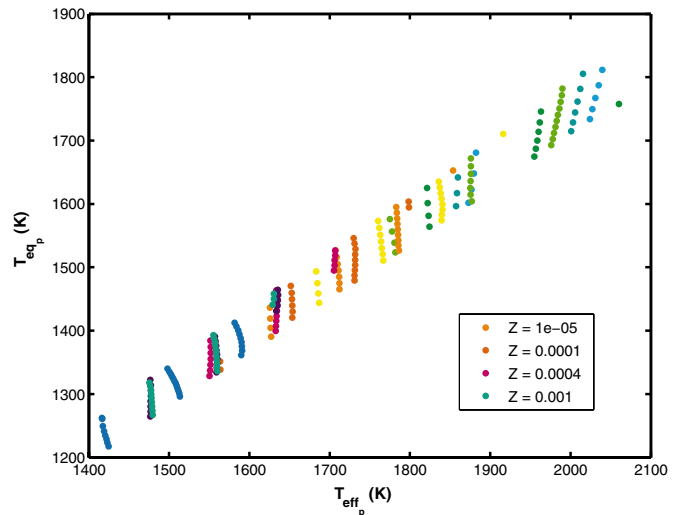
Figure 6. For the remaining valid dilution models (those that have parameters that overlap with stellar evolution tracks as shown in Figure 5), the equilibrium temperatures can be compared to the effective temperatures. To be of stellar nature, the values of T_{\text{eff},p} for each model would need to be much greater than the corresponding values of T_{\text{eq},p} (indicating that the companion is burning hydrogen). In this case, the temperatures are comparable and cannot be used to definitively rule out stellar blends, but this comparison may be useful to confirm other planet candidates.
