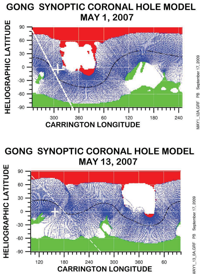
Fig. 4. Calculated coronal hole configurations according to GONG: Assuming a constant wind speed, we find the magnetic configuration at the source surface at the time, when a solar wind parcel left the Sun. Green denotes open field lines with positive polarity, red indicates negative polarity. The blue lines connect boundaries between open and closed magnetic field. The intercept of the black neutral line with the solar equator near the sub-terrestrial point (white cross) is taken for the location of the interface at the source. The parameter d , i.e., the slope of the interface at the source, has been derived from the white dashed line.
