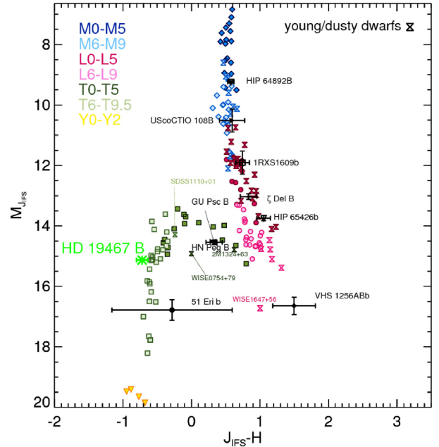
Figure 10. Absolute J magnitude versus J-H colour-magnitude diagram with the position of HD 19467 B that is indicated by a green asterisk. The positions of field M, L, and T dwarfs are also represented in different colours according to the spectral type. Black asterisks represent the positions of other substellar companions.
