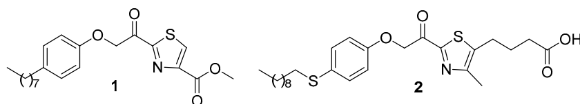
Figure 2. Examples of \alpha -ketothiazoles exhibiting anti-inflammatory properties.
