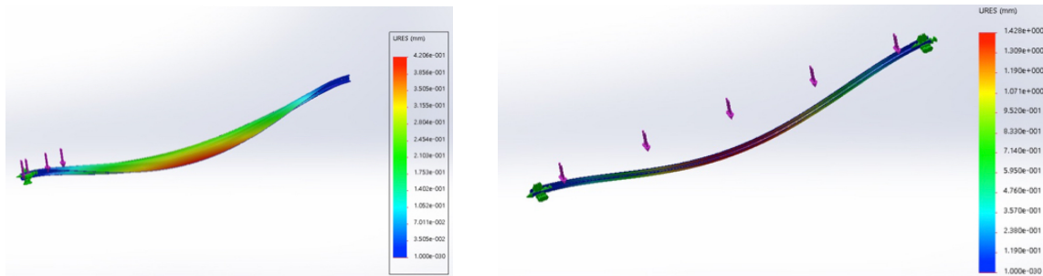
Figure 5.44. PD mechanical support analysis: rail deflection for the APA in the horizontal (left) and vertical (right) orientations.
