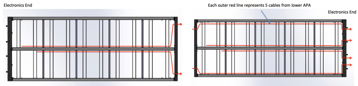
Figure 5.42. PD cable routing in APA frames: bottom APA (left) and top APA (right).
