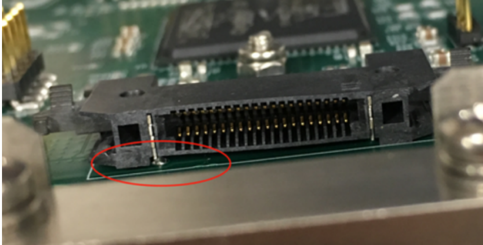
Figure 4.40. Image of a connector for the cold readout and signal cables, which has been lifted from the FEMB due to the presence of excess epoxy on the connection between the cold cables and the printed circuit board that acts as the “male” part of the connector.
