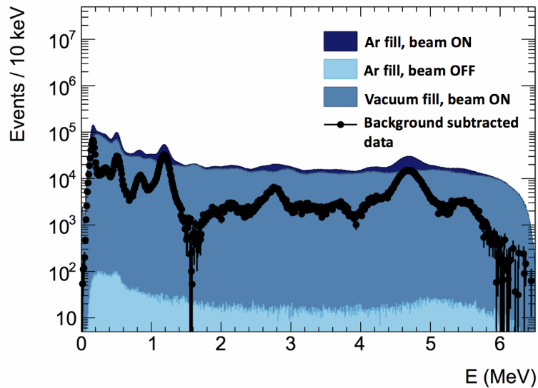
Figure 6.16. Energy spectra of individual \gamma clusters measured by ACED. Only events detected in the 0.02 eV to 0.04 eV neutron energy window are selected.
