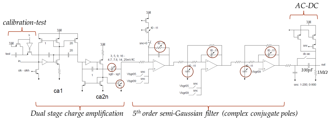
Figure 4.6. Channel schematic of LArASIC, which includes a dual-stage charge amplifier and a 5^{\text{th}} order semi-Gaussian shaper with complex conjugate poles. Circuits in red circles are programmable to allow different gain and peaking time settings.
