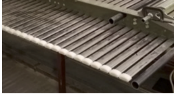
Figure 1.9. A section of the field cage, showing the extruded aluminum field-shaping profiles, with white polyethylene caps on the ends to prevent discharges.
