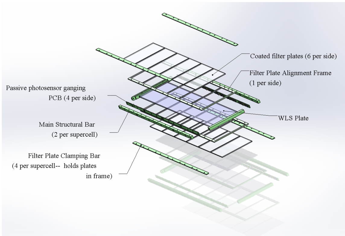
Figure 5.8. Detailed exploded view of X-ARAPUCA supercell. Note that components are designed to be cut from FR-4 G-10 sheets to simplify fabrication.
