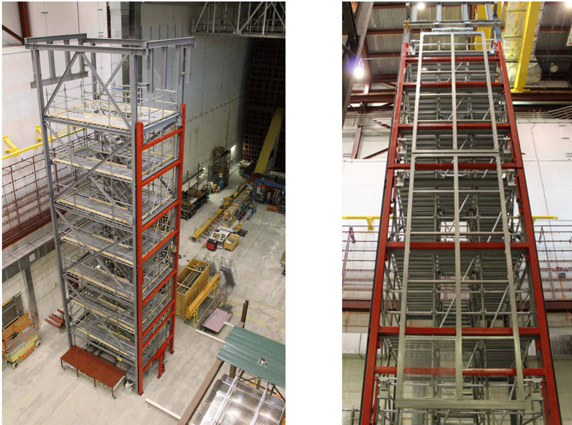
Figure 2.27. APA pair assembly and integration tests at Ash River.
