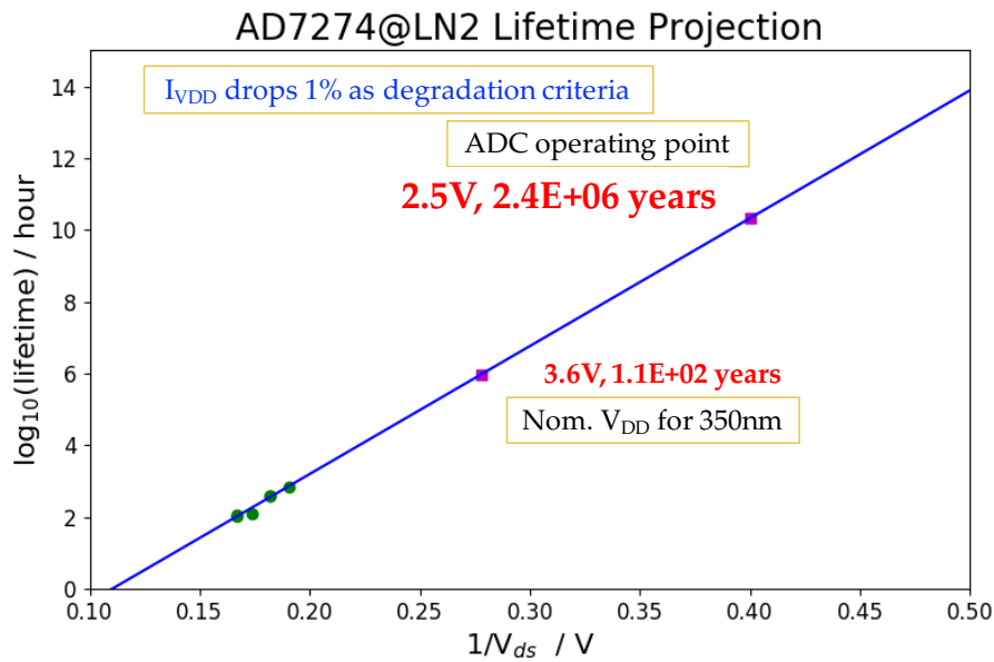
Figure 4.16. Lifetime projection of the COTS ADC AD7274 from the stress test with V_{DD} > 5V . The current drop of 1% on V_{DD} is used as the degradation criterion. With nominal operation voltage of 3.6 V for the 350 nm CMOS technology, the lifetime is projected to be more than 100 years. For SBND and the DUNE FD, the AD7274 will be operated at 2.5 V to add an additional margin; the expected lifetime is more than 1 \times 10^6 years.
