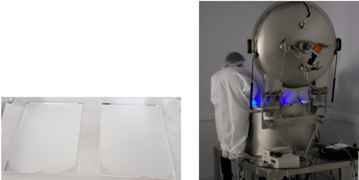
Figure 5.29. Coated dichroic filter plates (left) and UNICAMP thin film coating facility (right).
