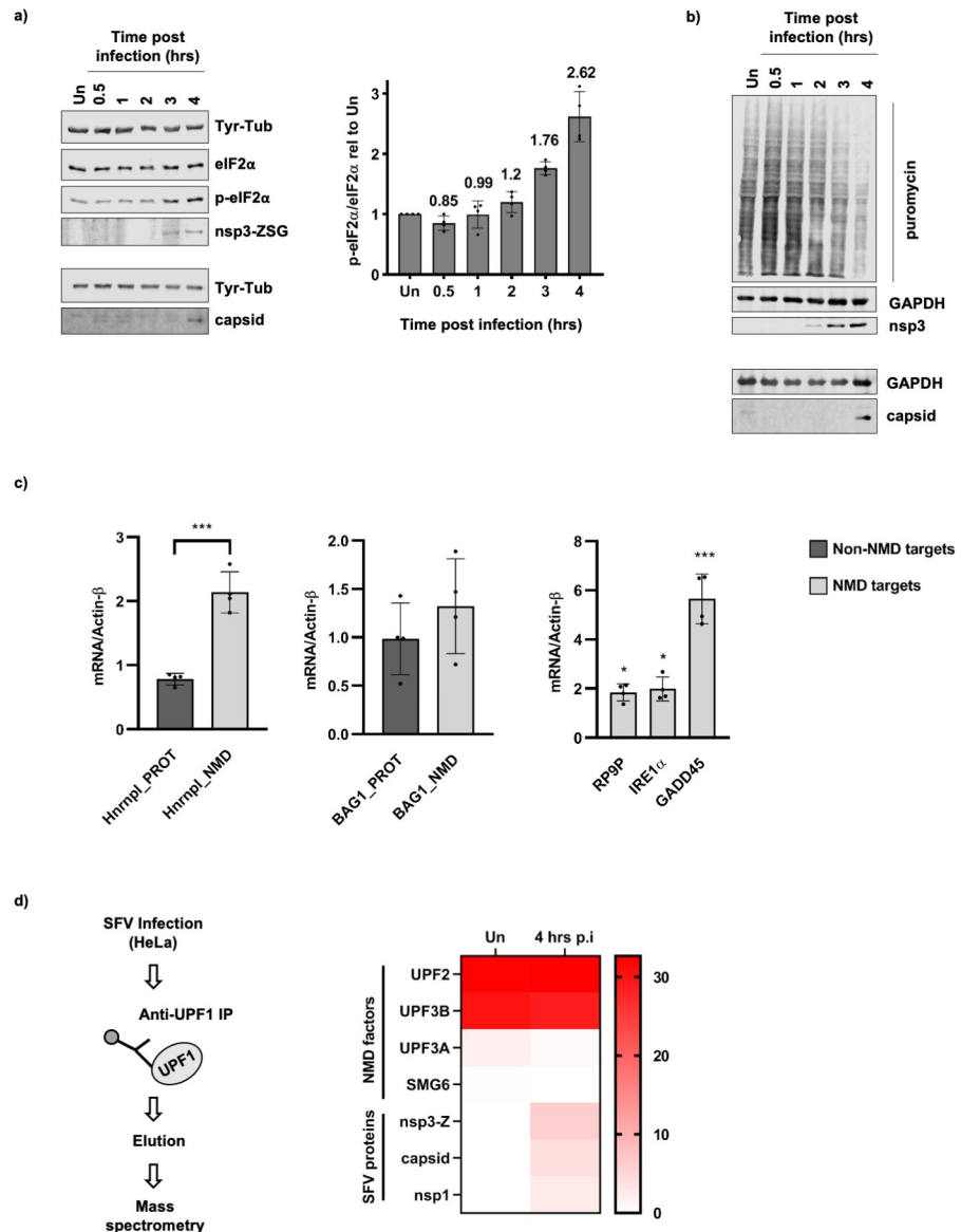
Fig 5. SFV infection inhibits translation and NMD, and UPF1 associates with SFV proteins. a , Representative western blots showing the induction of phosphorylated (p-)eIF2α versus eIF2α, as well as the accumulation of SFV proteins from the first ORF (nsp3-Z) and the second ORF (capsid) of the viral genome in a time course infection. SFV-ZSG infected HeLa cells were harvested at 0.5, 1, 2, 3 and 4 hours post infection. Uninfected cells (Un) were harvested at the 4 hour time point, Tyr-Tub was used as a loading control. The upper four panels represent a single blot that was cut and probed, while the lower two panels indicate a separate blot, on which the same set of samples was used. The bar graph (right) indicates the ratio of p-eIF2α/eIF2α relative to the uninfected sample, calculated from densitometry measurements of four western blots from independent time course infections. Mean values are shown above each bar (n = 4) and error bars reflect SD. b , Western blots showing the incorporation of puromycin into nascent polypeptides during a time course infection with SFV-ZSG (MOI = 10). GAPDH was used as a loading control. Nsp3-Z and capsid indicate the accumulation of SFV proteins during the infection. The upper 3 panels represent a single blot, while the lower two panels are from a separate blot analysing the same set of samples. c , RT-qPCR analysis showing mRNA levels relative to Actin-β of NMD targets (light grey bars) and non-NMD targets (dark grey bars) at 4 hours post infection, normalised to the uninfected control. Bar graphs display the mean ± SD (n = 4). Statistical significance was determined using unpaired, two-tailed t-tests, corrected for multiple comparisons using the Holm-Šidák method (GraphPad Prism v8.4.1), with alpha = 0.05. Asterisks indicate adjusted p values: p ≤ 0.05*, p ≤ 0.001***. d , Flow chart (left) depicting experimental approach for UPF1 immunoprecipitations (UPF1 IP) in uninfected (Un) and Infected (4 hours p.i.) cells, followed by mass spectrometry analysis to confirm UPF1 as an interactor of SFV proteins. Heat map (right) showing the abundance as % of the UPF1 bait for NMD factors and SFV proteins detected by mass spectrometry in the UPF1 eluate samples. Normalised spectral abundance factor (dNSAF) values were used.
