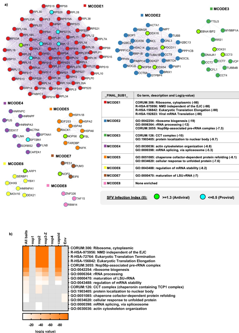
Fig 4. SFV interactors are highly enriched for GO terms related to translation, NMD and ribosome biogenesis. a, Protein-protein interaction enrichment analysis for the full list of SFV interactors was carried out using Metascape with the following databases: BioGrid, InWeb_IM and OmniPath. Densely connected network components were identified by applying the Molecular Complex Detection (MCODE) algorithm and the resultant MCODE networks are shown within the MCODE complexes (green and turquoise circles). In order to assign biological meanings to the MCODE networks, GO enrichment analyses were performed using the following sources: KEGG Pathway, GO Biological Processes, Reactome Gene Sets, Canonical Pathways and CORUM. All genes in the genome were used as the enrichment background. Between 1–4 GO terms were chosen to represent each MCODE network, with the relevant significance values depicted alongside them. b, Heat map comparing the significance of GO terms (chosen in a) among the different SFV baits. GO enrichment analysis was applied to the set of MCODE networks identified for each individual list (nsp1, nsp2, nsp3-Z, nsp4, capsid and Env), as well as for the merged list (All baits) and the significance values depicted in the heat map.
