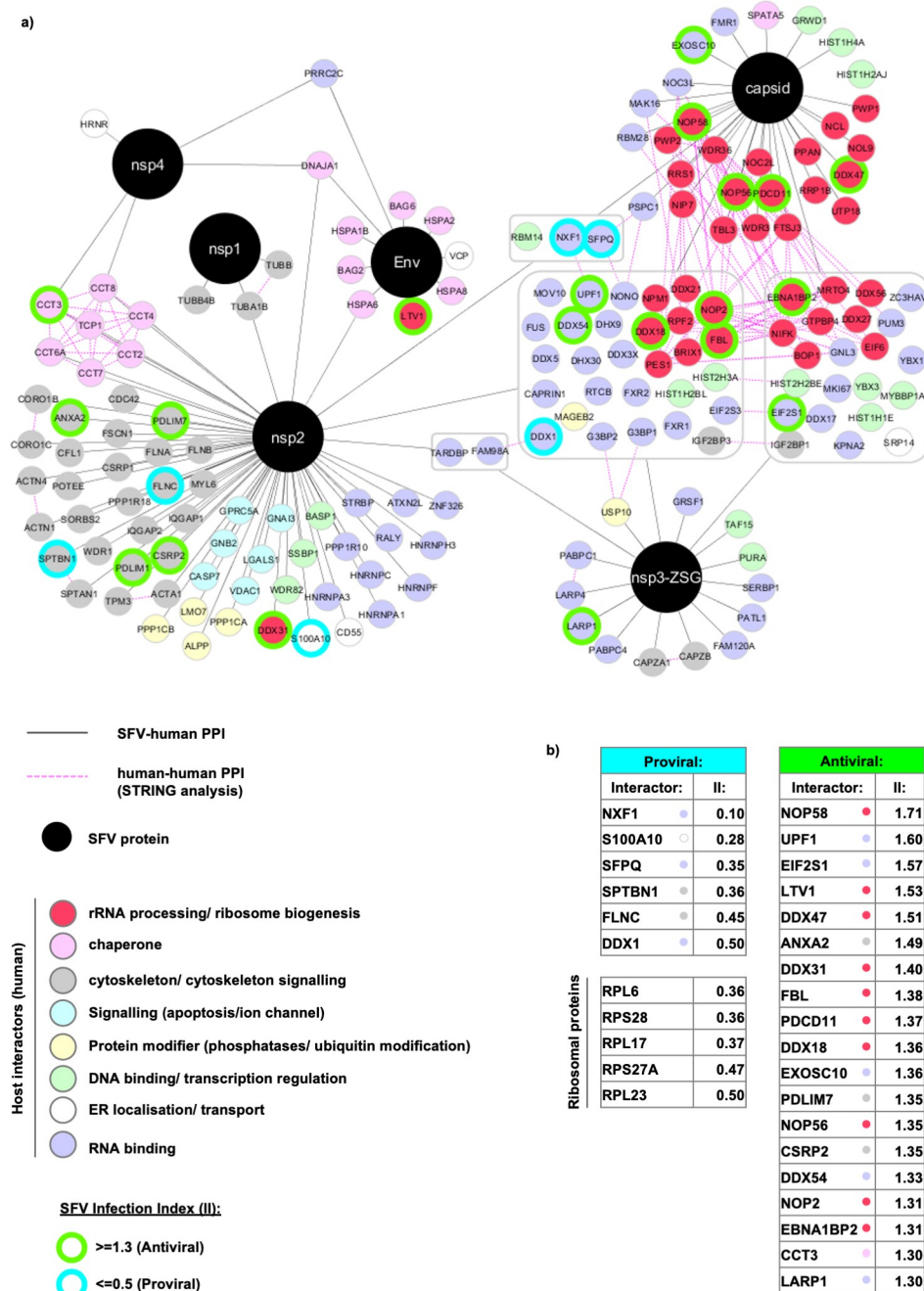
Fig 3. Network visualisation of the SFV-host protein interactome. a , In total, 174 host proteins are displayed. SFV proteins are depicted in black circles and host proteins are displayed in smaller colour-coded circles according to the key. SFV-host protein-protein interactions (PPI) are depicted with solid grey lines. Grey boxes reflect host proteins identified as interactors to more than one SFV protein. In these cases, the solid grey lines connect the grouped set of host proteins to the SFV proteins for which they were identified as interactors. Host-host PPI ascertained through STRING analysis are depicted with dashed pink lines. The host interactors were collected based on three independent biological replicates. For simplicity, ribosomal proteins (77) are shown separately in S3 Fig . SFV-host protein interactors identified through a genome-wide fluorescence microscopy based siRNA screen as exhibiting potential roles in SFV replication are additionally depicted with green and turquoise borders. A protein was defined as having a potential antiviral or proviral role if their Infection Index (II) values were \geq 1.3 or \leq 0.5 , respectively. b , Tables showing the II values of SFV-host interactors with potential proviral or antiviral roles.
