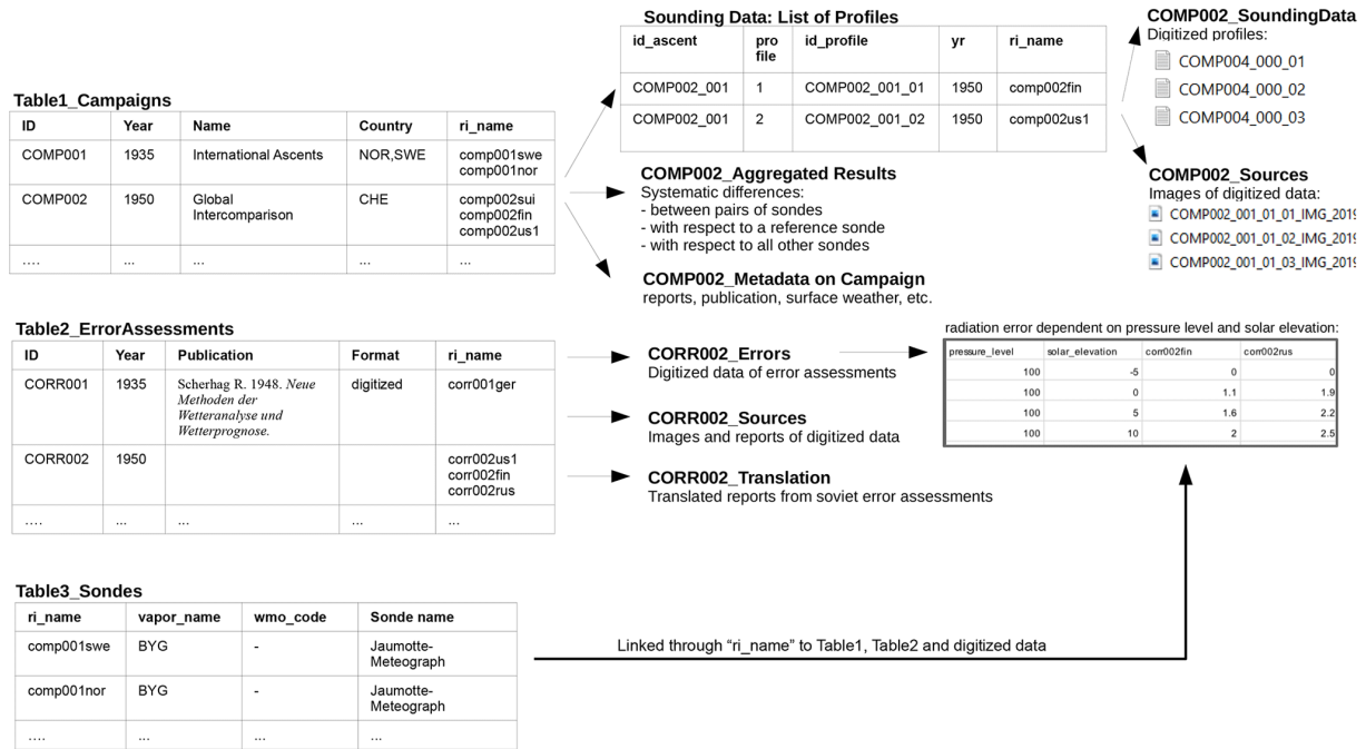
Figure 4. Schematic view of database structure based on the three tables for intercomparison campaigns, error assessments, and radiosondes. A common nomenclature links the different elements of the database, i.e., the digitized data files, the metadata, the source files, and the respective radiosondes.
