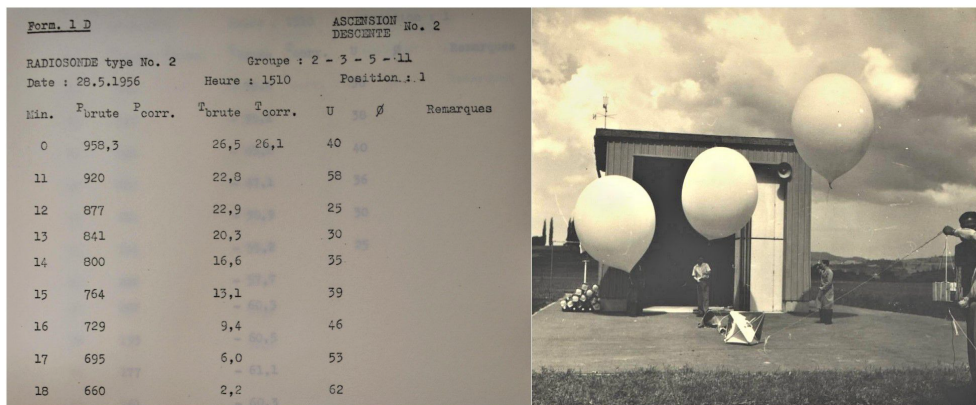
Figure 2. Left: sounding data from the 1956 campaign held in Payerne, Switzerland, from the archive of MeteoSwiss in Payerne (own image). Right: at the beginning of the campaign, soundings were performed with four radiosondes on a train of balloons (archive of MeteoSwiss). Within the course of the campaign this procedure changed to 13 radiosondes on a train of several balloons.
