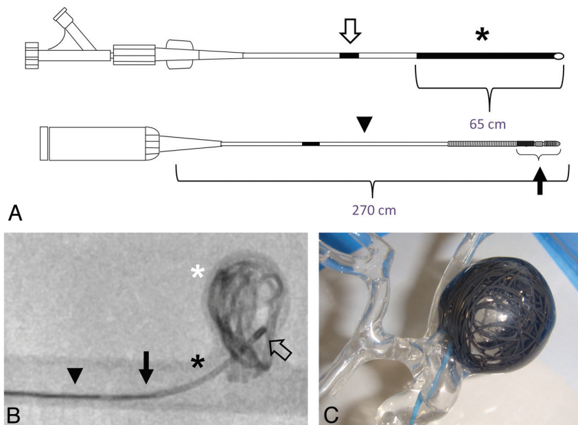
FIG 1. A, Schematic illustration of the polymeric coil system (above) and the delivery/detacher device (below). The coil system consists of a proximal shaft ( open arrow , ink marker) attached to a hemostatic valve and a distal 65-cm-long radiopaque polymeric strand with an outer diameter of 0.018 inch ( asterisk ). The delivery/detacher device (total length, 270 cm) is introduced through the hemostatic valve into the inner lumen of the coil system. The delivery/detacher device consists of the microwire ( arrowhead ) and the heater coil attached to its distal tip ( arrow ). B, Fluoroscopy of an in vitro silicon aneurysm model showing the radiopaque polymeric strand ( black asterisk ) within the microcatheter placed in the aneurysm (microcatheter tip, open arrow ) and its unfolded distal part within the aneurysm sac ( white asterisk ). Note the radiopaque section of the heater coil ( arrow ) at the distal tip of the delivery/detacher device ( arrowhead ) running within the coil strand. The polymeric strand can be detached at any point by advancing the radiopaque section of the heater coil at the level of the microcatheter tip and activating the thermal detachment. C, Photographic depiction of the silicon aneurysm model after introduction of the polymeric coil.
