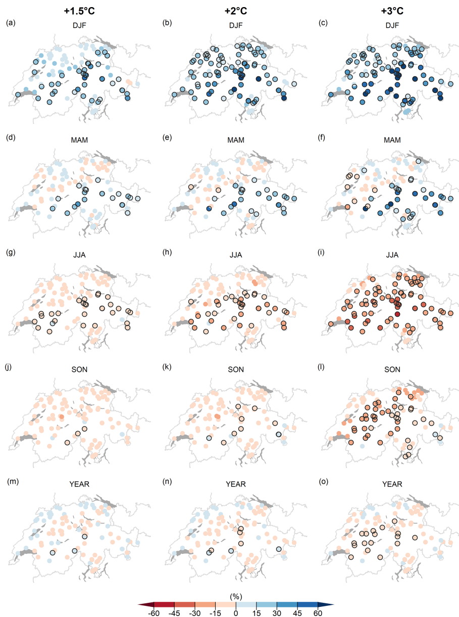
Figure 8. Multimodel median of seasonal and annual mean changes of runoff due to +1.5^{\circ}\text{C} (a, d, g, j, m), +2^{\circ}\text{C} (b, e, h, k, n), and +3^{\circ}\text{C} global warming for winter (a–c), spring (d–f), summer (g–i), autumn (j–l), and year (m–o). Black circles indicate catchments whose direction of change agrees across at least 90 % of the models.
