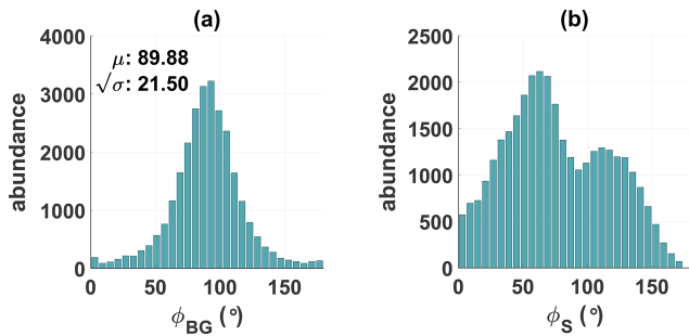
Figure 10. Histograms of the angle between the minimum variance direction and the background magnetic field (a) and the spacecraft-Sun connection line (b). The waves propagate predominantly perpendicular to the background field and at an angle \pm 65^\circ to the Sun.
