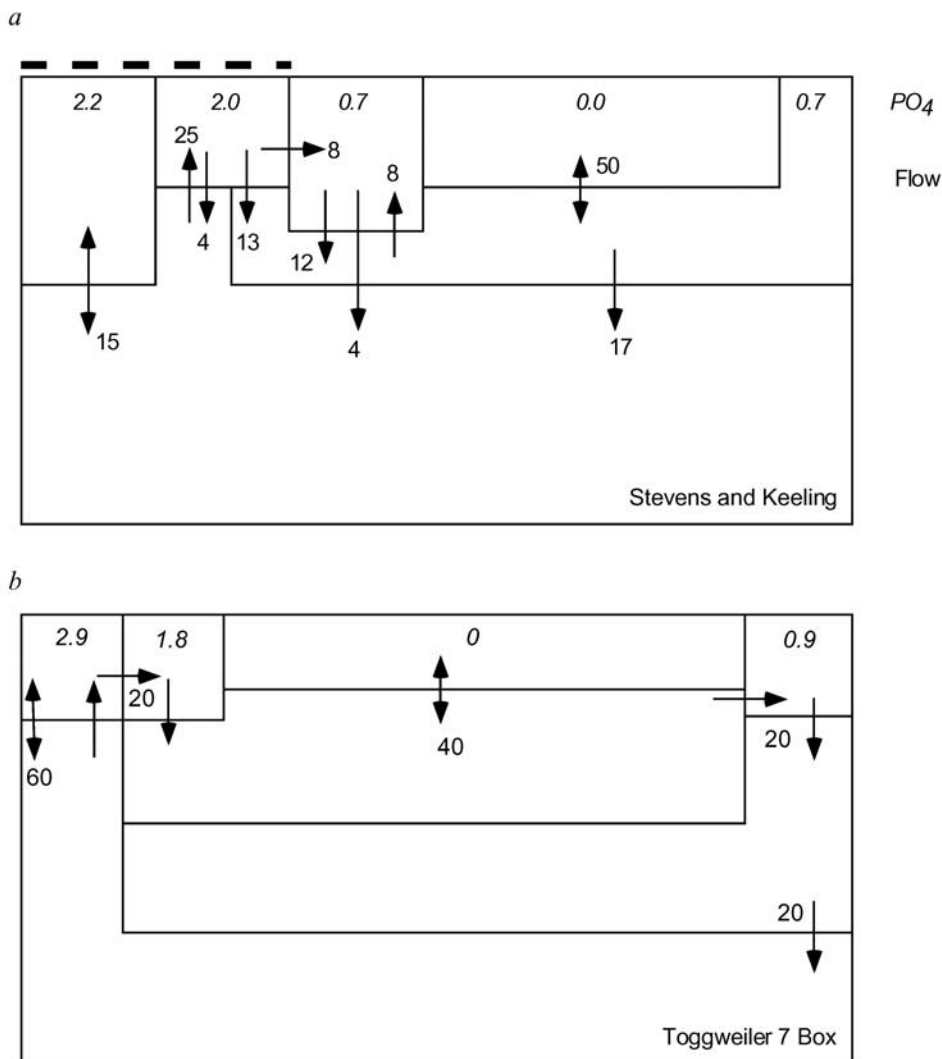
Figure 3. Schematic of box models from (a) Stevens and Keeling [2000] and (b) Toggweiler [1999]. Arrows represent water flows in Sverdrups, and italicized numbers show sea surface PO 4 concentrations. South is to the left.
