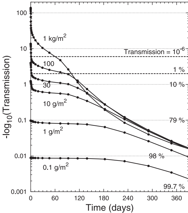
Figure 9. Evolution of transmission at \lambda = 0.55 \mu\text{m} through dust clouds with initial column densities of 10^{-4} , 0.001, 0.01, 0.03, 0.1, and 1 \text{ kg/m}^2 . Using equation (6), these amounts correspond to diameters of impacting asteroids of 0.5, 1, 2.2, 3, 4.8, and 10.3 km (solid lines). The dashed lines indicate the light level of full moonlight and a conservative estimate for the threshold of photosynthesis given by Toon et al. [1982]. Note that transmission may depend strongly on wavelength (Figure 6); therefore \lambda = 0.55 \mu\text{m} is not representative for the transmission of the total solar energy. Since the rate of coagulation increases with particle number density, the 1 \text{ kg/m}^2 cloud soon consist of larger particles than those in the 0.1 \text{ kg/m}^2 cloud. These high coagulation rates, leading to larger particles, increase the settling speed. Hence the transmission increases faster in the case of a 1 \text{ kg/m}^2 scenario than for the clouds with smaller initial column densities.
