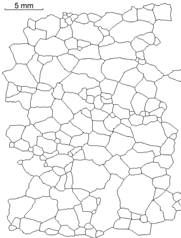
Figure 1. Example of a microstructure extracted from image analysis at a depth of 709 m. The vertical axis of the image corresponds to the true in situ vertical axis of the core.
