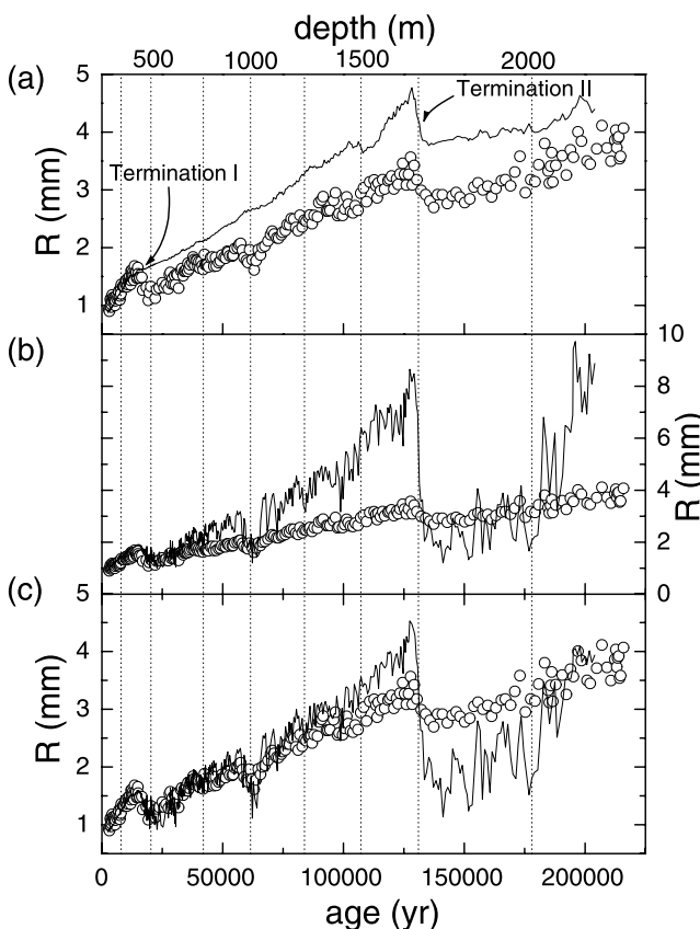
Figure 10. Pinning effect on the grain size evolution. Open circles show measured grain size \langle R \rangle . (a) Simulation taking into account the pinning effect of bubbles and clathrates (solid line). Terminations I and II are indicated by the arrows. (b) Simulation taking into account the pinning effect of dust particles (solid line). (c) Simulation taking into account the pinning effect of bubbles, clathrates, and dust particles (solid line).
