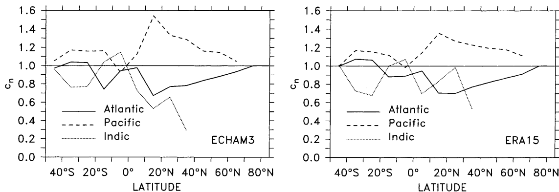
Fig. 13 Ratio of precipitation p_n into basin n (Atlantic, Pacific, Indic) to zonally averaged precipitation P as a function of latitude for the control run of ECHAM3 (left), and the ERA15 dataset (right)
