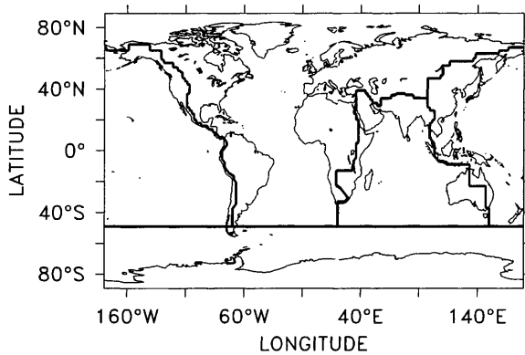
Fig. 12 Drainage basins for the Atlantic, Pacific, Indic and Southern oceans
