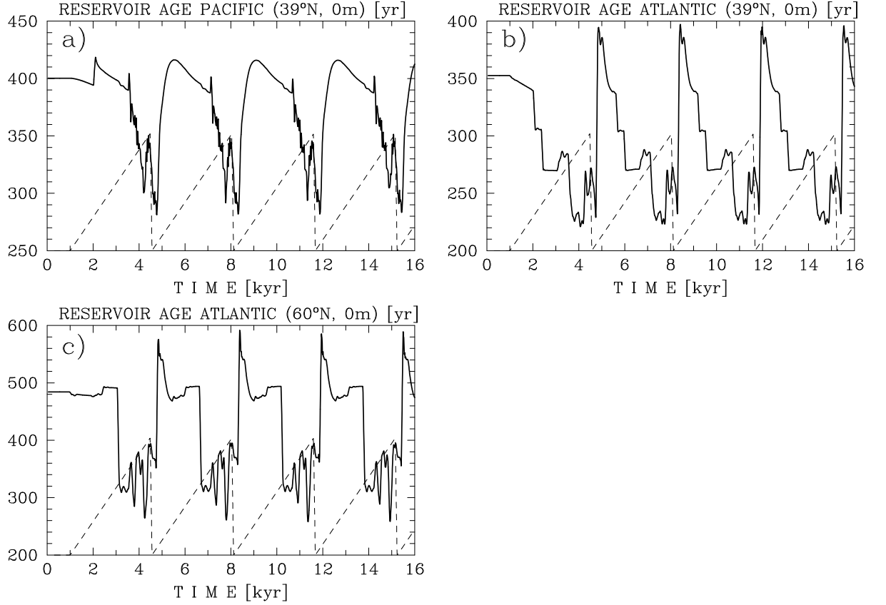
Figure 2: Evolution of the surface reservoir age in the Pacific at 39°N (a) and the Atlantic at 39°N (b), and 60°N (c). The age decreases during the cooling because of the reduced ventilation of the deep ocean. At the time of abrupt warming, deep waters that are depleted in radiocarbon are rapidly mixed to the surface increasing the surface reservoir age in the Pacific and mid-latitude Atlantic. There is a slight increase of the surface reservoir age in the Atlantic at 60°N during the cooling period. Remote regions may also be influenced by local convection changes, but the changes in the North Atlantic are rapidly communicated to all regions through the atmosphere. Note the scales for the reservoir ages at different locations.
