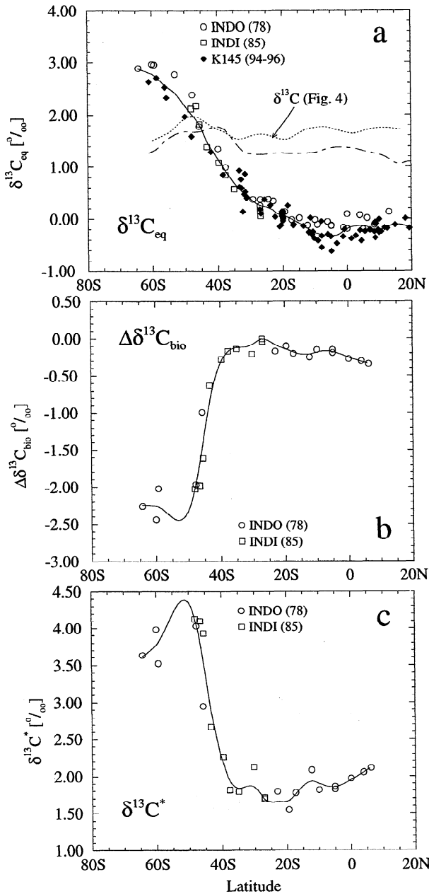
Figure 7. Same as Figure 5, but for the Indian Ocean. The spline fits through the \delta^{13}\text{C} observations shown in Figure 4a have been repeated in Figure 7a. In the case of INDO, \text{Alk} has been estimated from the global relationship of Gruber et al. [1996] in order to calculate \delta^{13}\text{C}_{\text{eq}} , \delta^{13}\text{C}_{\text{bio}} , and \delta^{13}\text{C}^* .
