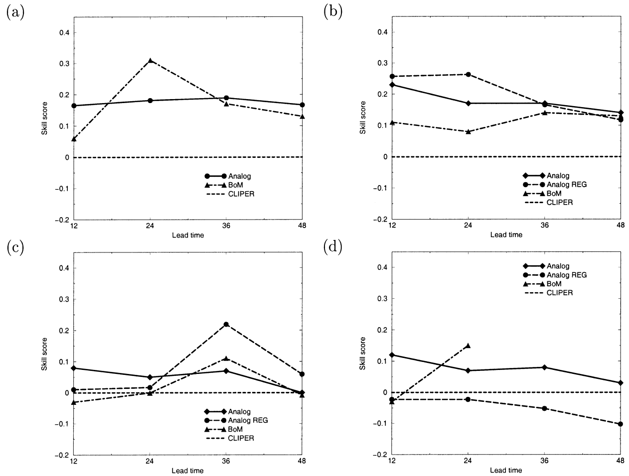
FIG. 5. Same as Fig. 4 but based on operational-track data: The skill of the adapted analog ensemble forecasts (1991–2000) is compared with the BOM official forecasts (triangles).
